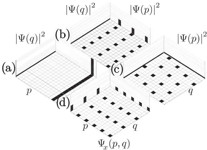
FIG. 4. The four classes of stabilizer states possible for odd nonprime d = 15 in terms of support: (a), (b) maximally supported in \mathcal{P} or \mathcal{Q} , (c) maximally supported in \mathcal{P} and \mathcal{Q} , and (d) not maximally supported in \mathcal{P} or \mathcal{Q} . The central grids denote the Wigner function \chi(\mathbf{p}, \mathbf{q}) for a stabilizer state with d = 15 . The projection of this state onto \mathcal{P} space is shown in the upper right [\chi(\mathbf{p})]^2 and the projection onto \mathcal{Q} space is shown in the upper left [\chi(\mathbf{q})]^2 .
