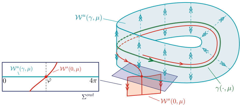
Fig. 6 Shown is a three-dimensional schematic of the gluing construction for systems with negative Floquet multipliers, where, for clarity, only W^u(\gamma(x, \mu), \mu) , the section \Sigma_{\text{out}} , and a heteroclinic orbit corresponding to an intersection of W^s(0, \mu) with W^u(\gamma(x, \mu), \mu) are shown. The setup is nearly identical to the orientable case, except that the phase coordinate \varphi \in [0, 4\pi] traverses \gamma twice
