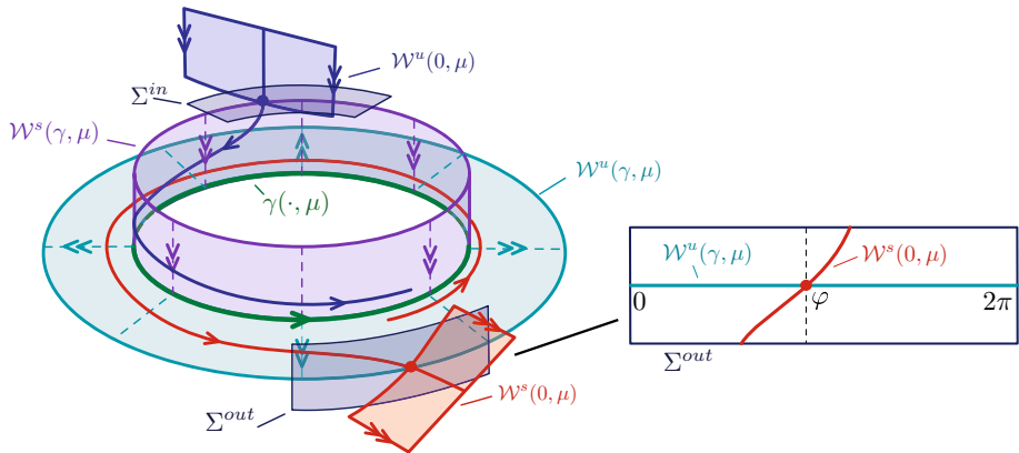
Fig. 4 Shown is a schematic of the geometry and the gluing construction near a periodic orbit with orientable stable and unstable manifolds without twists within the three-dimensional energy level set. Also shown are backs and fronts that correspond to intersections of W^u(0, \mu) with W^s(\gamma(x, \mu), \mu) and W^s(0, \mu) with W^u(\gamma(x, \mu), \mu) , respectively, and a zoom-in of the section \Sigma^{out} . Note that the sections \Sigma_{in} and \Sigma_{out} actually traverse all the way around the cylinders, but this is not drawn for clarity
