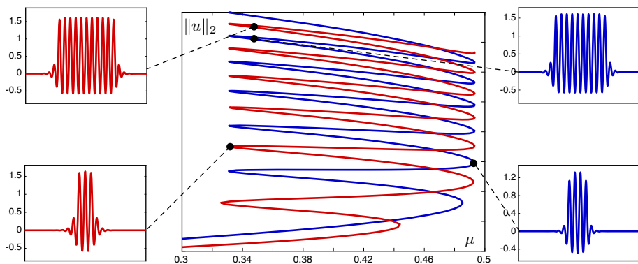
Fig. 14 Snaking of orientable localized rolls in the Swift–Hohenberg equation
