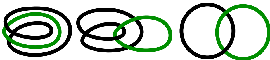
Fig. 11 From left to right: the boundary curve of a Möbius band (black) and its central circle (green) can be deformed to a pair of circles that have linking number one [1] (Color figure online)
