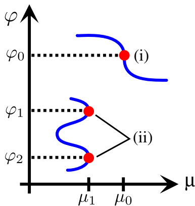
Fig. 9 Shown are two curve segments inside a sample set \Gamma = \{(\mu, \varphi) : G(\varphi, 0, \mu) = 0\} . The upper segment violates Hypothesis 8(i) at the filled circle with label (i) at which G_\varphi(\varphi_0, 0, \mu_0) = G_{\varphi\varphi}(\varphi_0, 0, \mu_0) = 0 : \Gamma is not locally a nondegenerate parabola near the point (\varphi_0, \mu_0) that corresponds to the vertical tangent. The lower segment violates Hypothesis 8(ii) at the two filled circles with label (ii) at which two vertical tangents arise at the same value of \mu so that G_\varphi(\varphi_j, 0, \mu_1) = 0 for j = 1, 2
