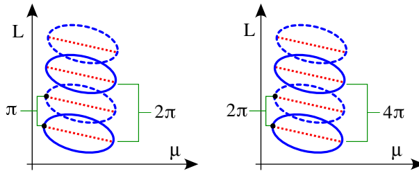
Fig. 8 Shown are sample bifurcation diagrams consisting of isolas in the orientable (left) and nonorientable (right) case: solid and dashed curves correspond to the branches \Gamma_{\text{sym}}^0 and \Gamma_{\text{sym}}^{\varphi_0} , respectively, of symmetric pulses with \varphi_0 = \pi in the orientable and \varphi_0 = 2\pi in the nonorientable case, while dotted curves correspond to branches of asymmetric pulses
