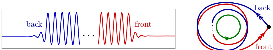
Fig. 2 The left panel shows the graphs of a back and a front as functions of space x . The interpretation of these patterns as heteroclinic orbits connecting the rest state to a periodic orbit is shown in the right panel. These heteroclinic solutions can be glued together to form a homoclinic orbit to the rest state that spends much of its trajectory near the periodic orbit, thus corresponding to a localized roll patterns
