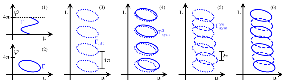
Fig. 7 Panels (1) and (2) show example sets \Gamma that are 1-loops and 0-loops, respectively. Panel (3) shows the set \Gamma_{\text{lift}} = \Gamma + (0, 4\pi\mathbb{Z}) (dotted) resulting from the 0-loop shown in panel (2), with the vertical axis variable \varphi replaced by L . Panels (4) and (5) show \Gamma_{\text{lift}} (dotted) together with the isolas \Gamma_{\text{sym}}^0 (solid) and \Gamma_{\text{sym}}^{2\pi} (dashed), respectively, that correspond to symmetric pulses; see Lemma 4.1. Panel (6) shows the sets \Gamma_{\text{sym}}^0 (solid) and \Gamma_{\text{sym}}^{2\pi} (dashed), whose union constitutes the full bifurcation diagram of symmetric pulses
