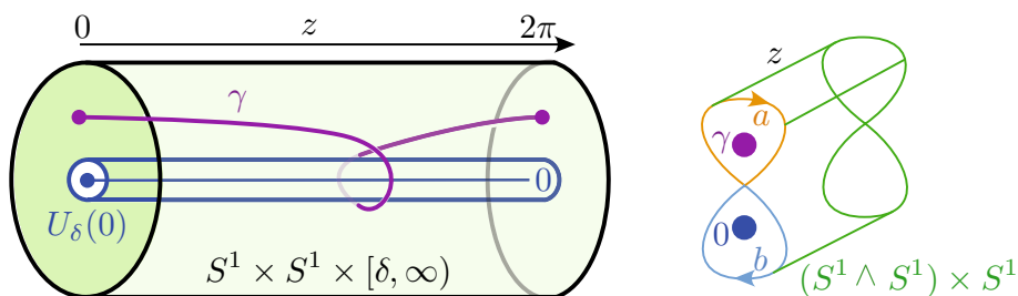
Fig. 13 Shown are the location of the periodic orbit \gamma in \mathcal{E}_\mu (left panel) and the generators a, b, z of the deformation retract (S^1 \vee S^1) \times S^1 of \mathcal{M} that form a basis of the fundamental group \pi_1(\mathcal{M})
