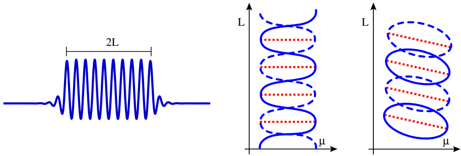
Fig. 1 Shown are the graph of a localized pattern with a roll plateau of length 2L as a function of space x (left panel) and schematic depictions of bifurcation diagrams that exhibit snaking (center panel) and disconnected closed curves (or isolas) (right panel): in the rightmost two panels, the solid and dashed curves correspond to the separate branches of symmetric pulses that have, respectively, a minimum and a maximum at their center, while the dotted curves correspond to disconnected branches of asymmetric pulses. Note that, throughout the paper, we will not indicate PDE stability in our bifurcation diagrams
