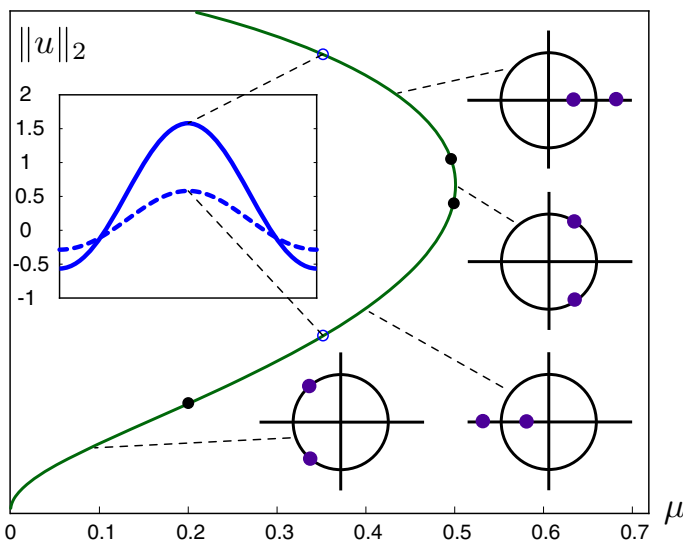
Fig. 12 Shown is the family of periodic orbits with zero energy emerging from \mu = 0 in the Swift–Hohenberg equation (1.1) with nontrivial Floquet multipliers indicated in the insets. Note that, for a range of values of \mu , there exist both orientable (positive Floquet multipliers) and nonorientable (negative Floquet multipliers) periodic orbits. At the value of \mu = 0.35 , the profiles of the periodic orbits are shown: the orientable and nonorientable orbits are shown in solid and dashed blue, respectively (Color figure online)
