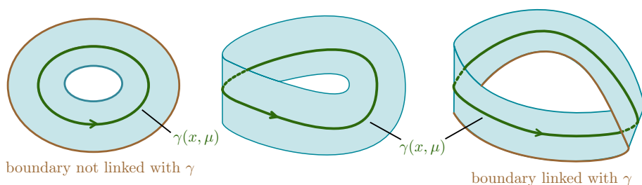
Fig. 3 Shown are the periodic orbit \gamma(x, \mu) and its two-dimensional unstable manifold within the three-dimensional zero level set of the energy. The three panels indicate the cases where, from left to right, the unstable manifold is orientable without twist (thus homeomorphic to a cylinder), nonorientable with a half twist (hence homeomorphic to a Möbius band), and orientable with a full twist (again homeomorphic to a cylinder). Note that, in contrast to the case without twist, the boundary of the rightmost unstable manifold forms a nontrivial knot with the periodic orbit
