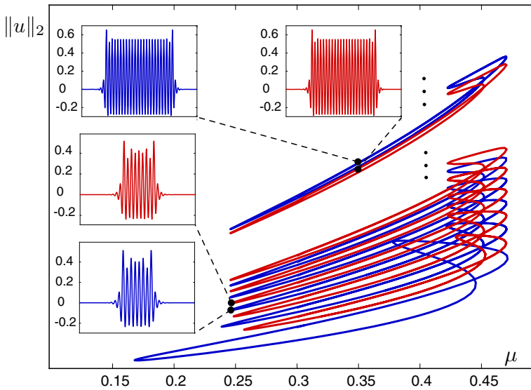
Fig. 15 Isolals of nonorientable localized rolls in the Swift–Hohenberg equation
