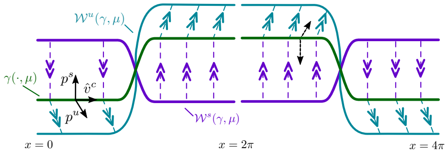
Fig. 5 Shown is an illustration of the stable and unstable manifolds of the periodic orbit \gamma in the nonorientable case: the vectors in black represent p^s(x, \mu) and p^u(x, \mu) , and it is indicated how they change direction after 2\pi time units. Considering the phase in the interval [0, 4\pi] allows us to match the vector directions and visualize the stable and unstable manifolds of the periodic orbit as two Möbius bands glued together
