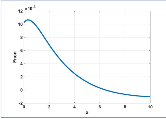
Fig. 12. The polynomial fit of the identified electrostatic force at 1 V Volt as the gap varies. This force profile presents the equivalent electrostatic force of the lumped model. The force and the gap are non-dimensional.
