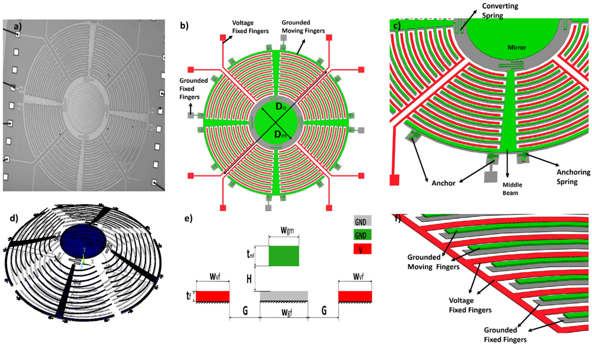
Fig. 1. Presented mirror model. (a) Microscope image of whole device. (b) Top view of 3D model. (c) Isometric view of the 3D Model. (d) The first mode shape of the system obtained from ANSYS. (e) A unit cell of the repulsive actuator configuration. The dimensions are given in Table 1. (f) Closer view of the finger configuration in the 3D model.
