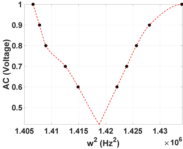
Fig. 10. Transition curve of principal parametric resonance for V_{DC}=40 V. Markers indicate measured data and the lines show the data interpolation.
