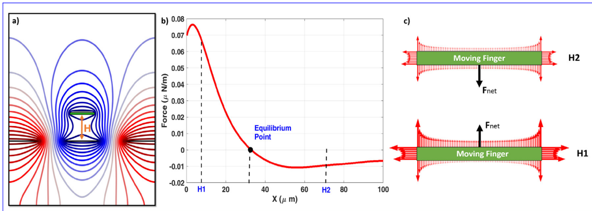
Fig. 2. Finite element simulation using COMSOL package including (a) electric field contours, (b) force profile for the unit cell as the vertical gap H varies at V=1\text{ V} , (c) electrostatic force distribution on the moving finger at the vertical distance of H_2 (top figure) and H_1 (bottom figure). For the bottom figure, the net force on the moving finger is upward (repulsive). For the top figure, the net force is downward (attractive).
