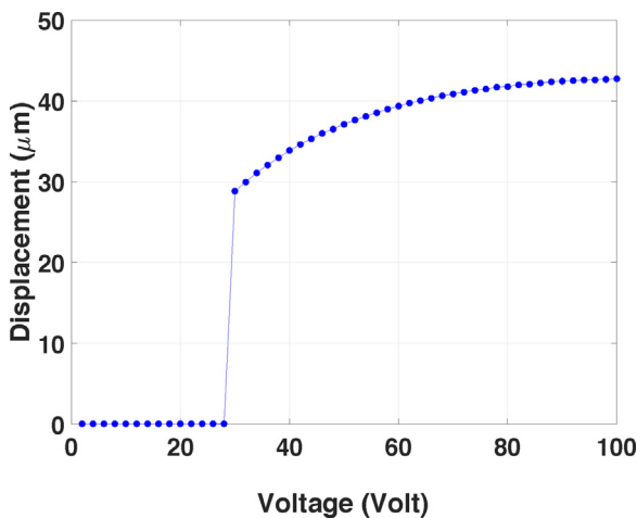
Fig. 3. Static deflection versus DC voltage.
