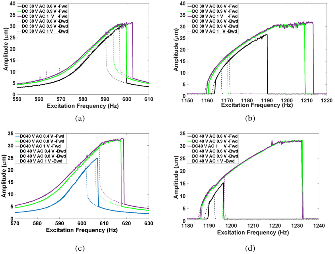
Fig. 9. Measured frequency response curve as AC voltage varies for (a) fundamental resonance for DC 38 V, (b) principal parametric resonance for DC 38 V, (c) fundamental resonance for DC 40 V, (d) principal parametric resonance for DC 40 V.
