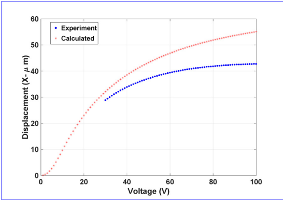
Fig. 13. Comparison of the static deflection results from simulations and experiments. For the simulations, the force is calculated from the 2D finite element force profiles.
