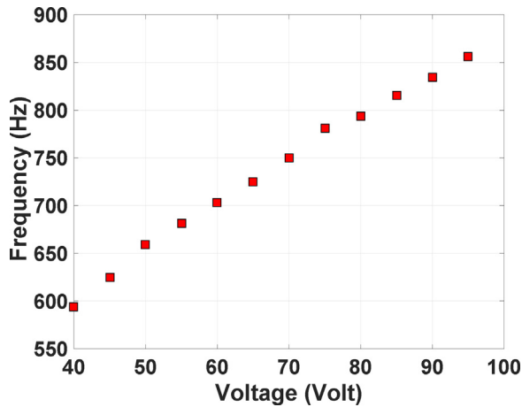
Fig. 5. Linear natural frequency obtained for different DC loads at 120 mTorr. Red squares indicate measured values.
