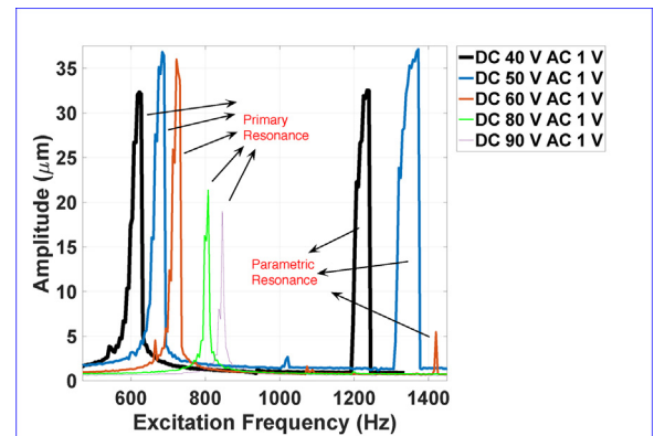
Fig. 6. Experimental frequency curves as DC voltage varies from 40 V to 90 V at AC voltage is 1 V at 35 mTorr.
