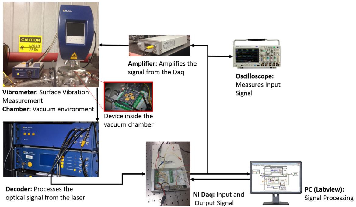
Fig. 4. Experimental setup with Doppler vibrometer.
