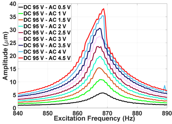
Fig. 7. Experimental frequency response curve when DC is 95 V and AC varies from 0.5 to 4.5 V. The pressure of the vacuum chamber is 35 mTorr for this case.
