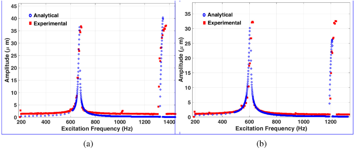
Fig. 14. Comparison of simulated and measured frequency responses at (a) V_{dc}=50 V and V_{ac}=1 V, (b) V_{dc}=40 V and V_{ac}=1 V.
