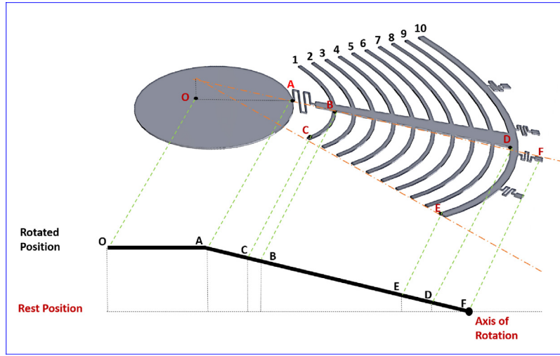
Fig. 11. Schematic of the mirror and beams in one set of actuators once the mirror lifts.
