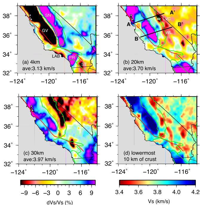
Fig. 6. Vs tomography maps from the Rayleigh wave Monte Carlo inversions at the depths of (a) 4, (b) 20, and (c) 30 km, respectively, plotted as perturbations relative to the regional average across the entire research area. The thick white line in (b) denotes the Long Valley Caldera according to Seccia et al. (2011). The two thick black lines in (b) show the locations of the transects in Fig. 7. (d) Vs averaged within the lowermost 10 km of the Moho, plotted as absolute values. The local Moho depth is defined by the average of the posterior distributions of crust thickness from the MCMC inversion (Fig. S1b). Other lines are as in Fig. 2. Abbreviations: GV—Great Valley, SN—Sierra Nevada, LAB—Los Angeles Basin, PR—Peninsula Ranges, ST—Salton Trough, LVC—Long Valley Caldera, WL—Walker Lane.
