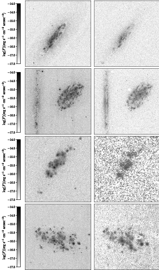
Fig. 8. Comparison of the H\alpha images of the galaxies NGC4313 (SA(rs)ab:edge-on), NGC 4298 (SA(rs)c) and NGC4302 (Sc:edge-on), IC3239 (Sm) and IC 3365 (Im) obtained by VESTIGE ( left column, from top to bottom ) to those obtained with a \sim 900 s on-band exposure on the 2.1 m telescope at San Pedro Martir (NGC 4313, IC3239, IC3365; Gavazzi et al. 2003b) or a 4000 s exposure on the 0.9 m telescope at Kitt Peak (NGC 4298 and 4302; Koopmann et al. 2001) ( right ).
