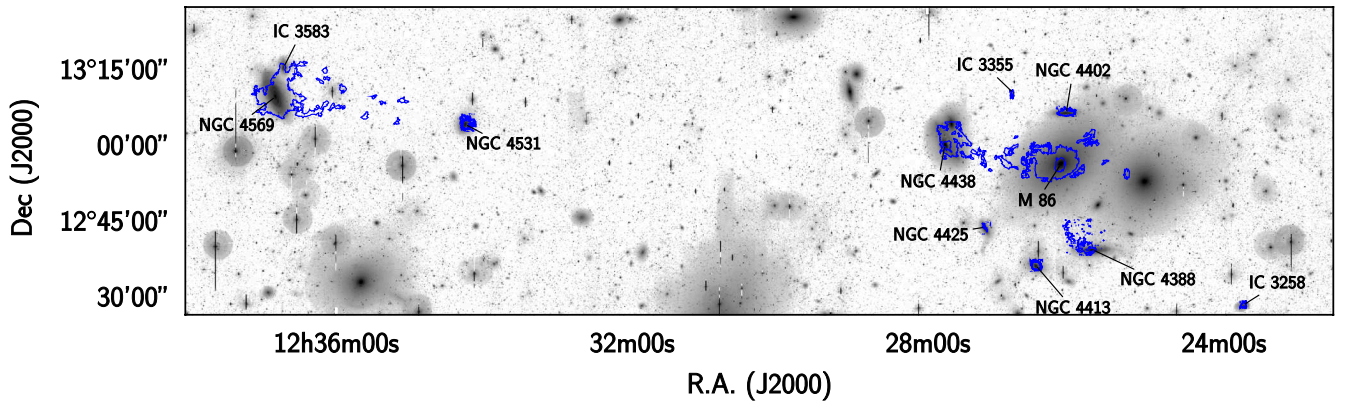
Fig. 10. Continuum-subtracted H\alpha contours (blue) overplotted on the r -band image (grey) of the 4 \times 1 \text{ deg}^2 ( 1.1 \times 0.3 \text{ Mpc}^2 ) strip of the core of the cluster north of M87. Given that the survey still does not reach its full sensitivity, contours are measured at different surface brightness levels: \Sigma(H\alpha) \approx 10^{-18} \text{ erg s}^{-1} \text{ cm}^{-2} \text{ arcsec}^{-2} for NGC 4569 and IC 3583 (from Boselli et al. 2016a), \Sigma(H\alpha) \approx 3 \times 10^{-18} \text{ erg s}^{-1} \text{ cm}^{-2} \text{ arcsec}^{-2} for IC 3355, NGC 4388, and NGC 4531, and \Sigma(H\alpha) \approx 6 \times 10^{-18} \text{ erg s}^{-1} \text{ cm}^{-2} \text{ arcsec}^{-2} for M86, IC 3258, NGC 4402, NGC 4413, NGC 4425, and NGC 4438.
