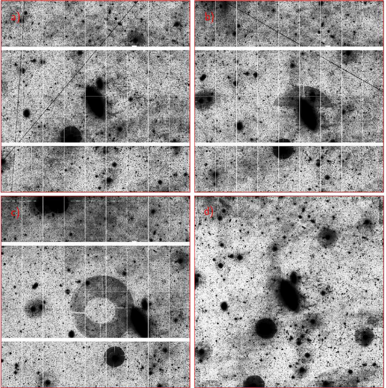
Fig. 4. Panels a–c: megaCam images of the galaxy NGC 4569 obtained during three different pointings reduced using the standard Elixir pipeline. A prominent ghost due to the reflection of a star is evident in two of them ( panels b and c ). Given their different position on the frame, the ghosts are efficiently removed after stacking seven independent frames reduced using Elixir-LSB ( panel d : the grid pattern in the periphery of this frame is due to undersampled regions).
