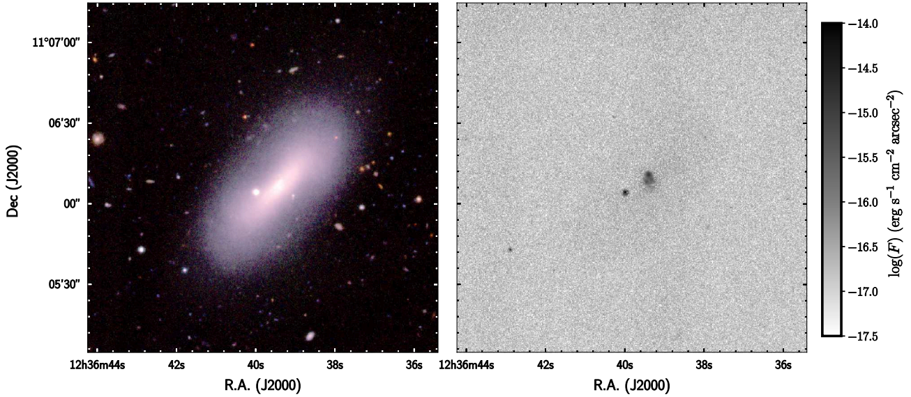
Fig. 11. NGVS ugi rgb colour image ( left ) and the VESTIGE continuum-subtracted H\alpha image of the dwarf spheroidal galaxy (dS0(8): Binggeli et al. 1985) IC 3578 (VCC 1684). The H\alpha image shows the presence of a few compact HII regions in the nucleus of the galaxy, witnessing an ongoing nuclear star forming activity.
