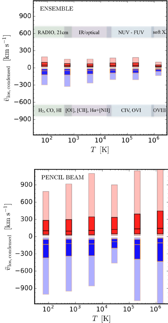
Figure 3. Ultra high-resolution (0.8 pc) simulation following the multiphase CCA rain for 100 Myr in a central massive galaxy (analogue of Fig. 2): luminosity-weighted LOS velocity (line shift) of the multiphase gas for the 6 phase bins. The bars indicate the mean and 1-2 standard deviation (dark to light) in log space of the underlying points, which are tracked every 1 Myr for each of 3 random lines of sight. We note the driven hot keV plasma (not shown) has a null velocity shift with negligible error. Blue/red colors denote blue-/redshifted lines compared with the galactic systemic velocity. The line shift magnitudes are best fitted by lognormal distributions. Top: The ensemble gas detections show on average a small line shift, with average magnitude less than a few tens \text{km s}^{-1} , and thus would sometimes appear consistent with the galactic dynamics. Bottom: The pencil-beam detections, on the other hand, show substantially larger line shifts of the order of several 100 \text{ km s}^{-1} , with a large scatter ( \sim 0.5 dex).
