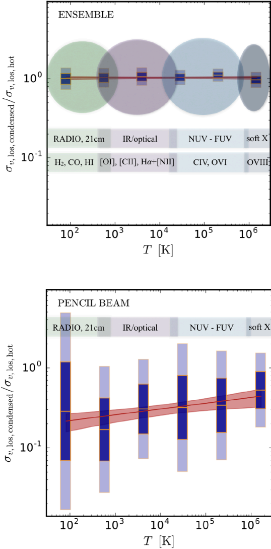
Figure 2. Ultra high-resolution (0.8 pc) simulation following the multiphase CCA run for 100 Myr in a central massive galaxy: luminosity-weighted LOS velocity dispersion (line broadening) of the multiphase gas (from ionized to molecular gas, 6 bins with 0.9 dex width) normalized to the hot plasma ( > 5 \times 10^6 K) turbulence. The latter (not shown) is continuously driven with a stable one-dimensional velocity of the order of 100 \text{ km s}^{-1} . The bars indicate the mean and 1-2 (dark to light) standard deviations in log space of the underlying points, which are tracked every 1 Myr. Each point is computed as the median out of 5 random lines of sight. We note, for a Gaussian line, \text{FWHM} = 2\sqrt{2 \ln 2} \sigma_{v,\text{los}} . The brown line and bands show the best-fit linear regression (in log space) and associated 99% confidence levels (with 10^5 iteration bootstrapping) for the computed points over the 6 phases. Top: Ensemble-beam detection in the projected radial range 0.5–15 kpc. The correlation is tight throughout the multiphase condensation cascade, thus we can use the ensemble detection as robust proxy for the turbulence in the hot gas (or between other phases). Bottom: Same as above but for a pencil-beam ( R \lesssim 25 pc) observation. The velocity dispersion decreases significantly, in particular for the cold phase, thus narrow lines are expected to be detected frequently with this technique. The scatter increases substantially, implying that systems observed with a pencil beam (e.g., through the AGN backlight or CO emission) can also display a broad component. The narrower component is typically associated with inner denser clouds, which have experienced several collisions and are being funneled toward the supermassive black hole.
