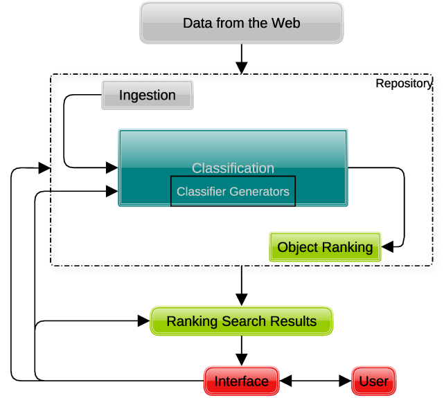
Figure 1: HYBRID.AI Architecture
