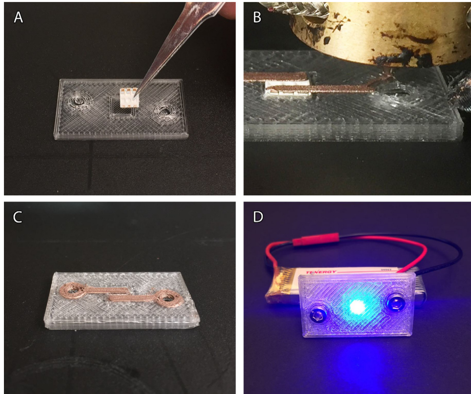
Fig. 7. Embedded LED as an example of interfacing with off-the-shelf components. (A) Printing process is paused and LED is placed into a cavity before resuming the print. (B) Conductive traces are printed on top of the LED contacts, and (C) the LED component is fully embedded. (D) Screw terminals are used to attach a battery to the Electrifi traces and light the LED.
