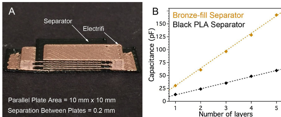
Fig. 5. (A) Half-slice view of the printed five-layer parallel plate capacitor with black PLA separator. (B) Plot of capacitance versus the number of stacked parallel plate layers for two different separator materials.
