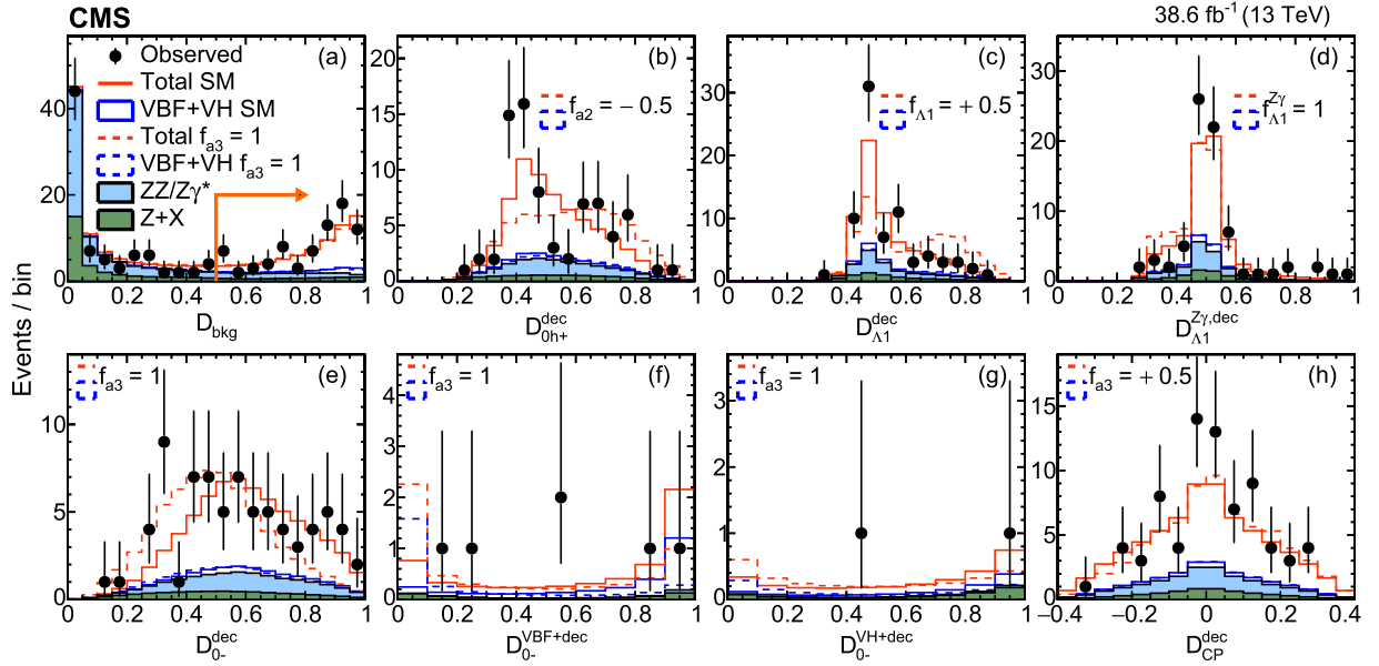
Fig. 2. Distributions of \mathcal{D}_{\text{bkg}} (a) for all events in Run2; \mathcal{D}_{0h+} (b), \mathcal{D}_{\Delta 1} (c), \mathcal{D}_{\Delta 1}^{Z\gamma} (d), \mathcal{D}_{0-} (e), and \mathcal{D}_{CP} (h) for the untagged and 2015 events; \mathcal{D}_{0-} in the VBF-jet (f) and VH-jet (g) categories. The arrow in (a) indicates the requirement \mathcal{D}_{\text{bkg}} > 0.5 , used to suppress background on all other plots. Points with error bars show data and histograms show expectations for background and signal, as indicated in the legend in (a). The dashed lines show expectations for BSM hypotheses, as indicated in the individual legends.
