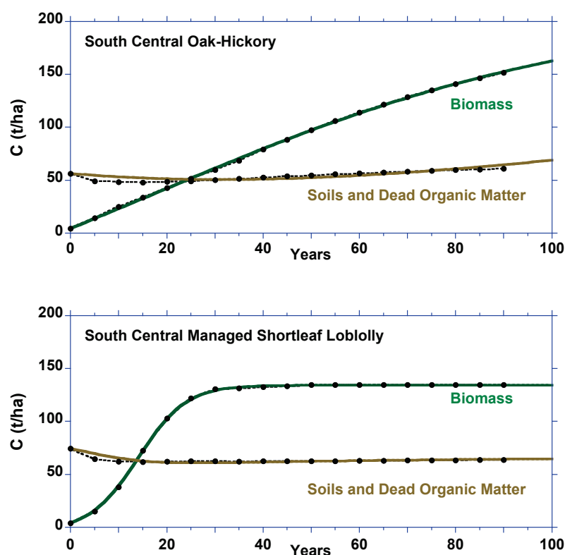
Figure 2. Growth curves showing carbon density ( \text{tC ha}^{-1} ) for oak-hickory (top) and managed shortleaf loblolly pine plantations (bottom) in the south-central US, comparing Smith et al (2006) growth curves (dashed lines with data points) to the model (solid lines), with best-fit parameters. Supplementary figure S2 and tables S2–S3 show results for all forest types estimated.
