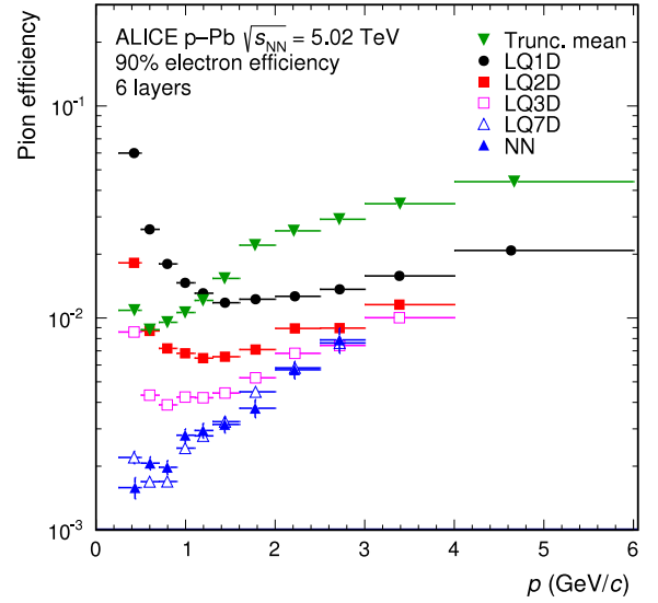
Fig. 43. Pion efficiency (for 90% electron efficiency) as a function of momentum for the truncated mean, LQ1D, LQ2D, LQ3D, LQ7D and NN methods. The results are from p–Pb collisions at \sqrt{s_{NN}} = 5.02 TeV and for tracks with signals in six layers.
