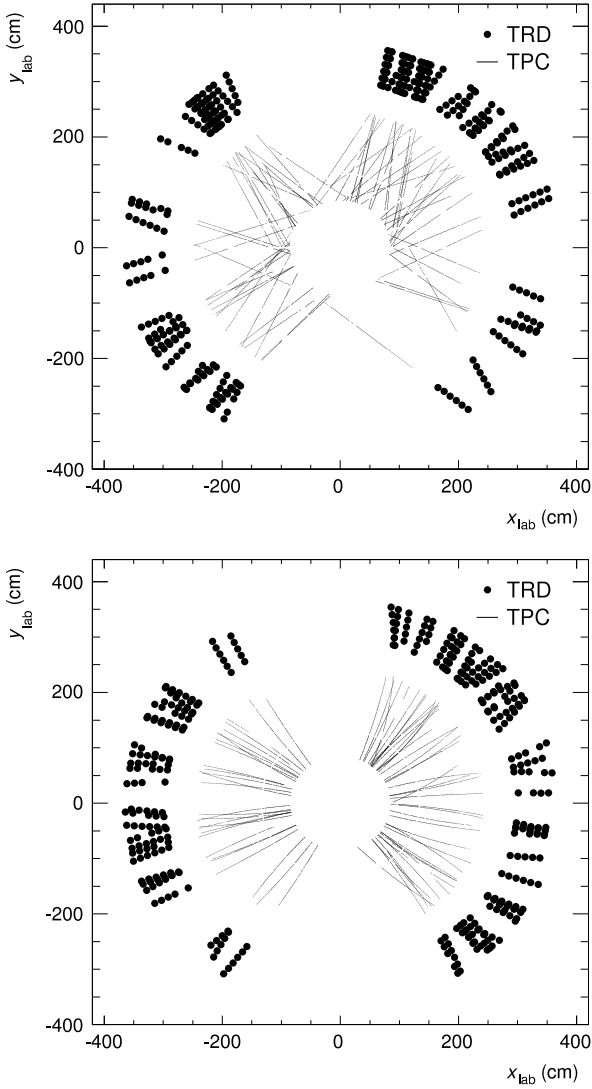
Fig. 28. Top: Cosmic-ray tracks with at least 100 TPC clusters and 5 TRD layers, recorded without magnetic field, used for the relative rp alignment of the TRD chambers within stacks (internal alignment). Bottom: Charged-particle tracks with at least 100 TPC clusters and 4 TRD layers from pp collisions at \sqrt{s} = 8 TeV, used for the alignment of the TRD with respect to the TPC (external alignment). Both figures show data from 2012 (setup with 13 supermodules).
