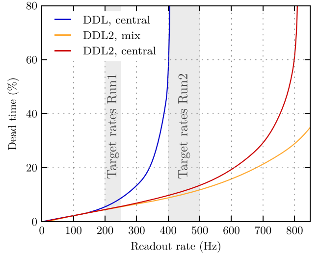
Fig. 16. Simulation of the dead time as function of the read-out rate in Pb-Pb collisions for the effective DDL bandwidth in Run 1 (DDL) and Run 2 (DDL2). The simulation assumes a 5% L1/L0 accept ratio and no L2 rejects. The scenarios central and mix correspond to an event size of 470 kB and 310 kB per supermodule, respectively, mimicking thus different event multiplicities.
