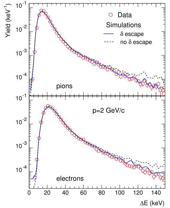
Fig. 6. Distributions of the ionisation energy loss of pions and electrons with momenta of 2\text{ GeV}/c . The symbols represent the measurements obtained at the CERN PS with prototype read-out chambers that were smaller in overall size (active area 25\text{ cm} \times 32\text{ cm} ) but otherwise similar in construction to that of the final detector. The lines are simulations accounting (continuous line) or not (dashed line) for the long range of \delta -electrons as compared to the chamber dimensions. Figure taken from [48].
