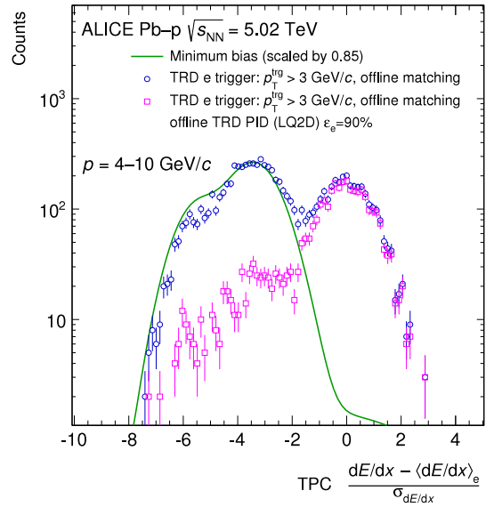
Fig. 58. Electron selection for triggered data with and without the TRD offline PID (see Section 11) in Pb-p collisions at \sqrt{s_{NN}} = 5.02 TeV. Electrons from photon conversions in the detector material were rejected by matching the online track with a track in the TPC. The corresponding distribution for minimum-bias data, scaled to the maximum of the distribution of the triggered data sample, is shown to visualise the TRD trigger capability to enhance electrons.
