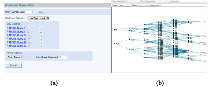
Figure 4: (a) Screen to select a workload for contention analysis. (b) Screen to perform a time-series analysis of iQ-Graph.
