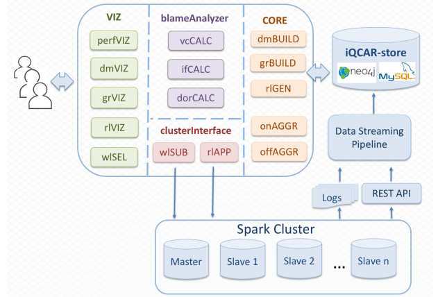
Figure 2: iQCAR Architecture
