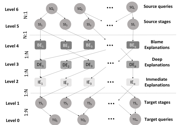
Figure 1: iQC-Graph with three levels of explanations.
