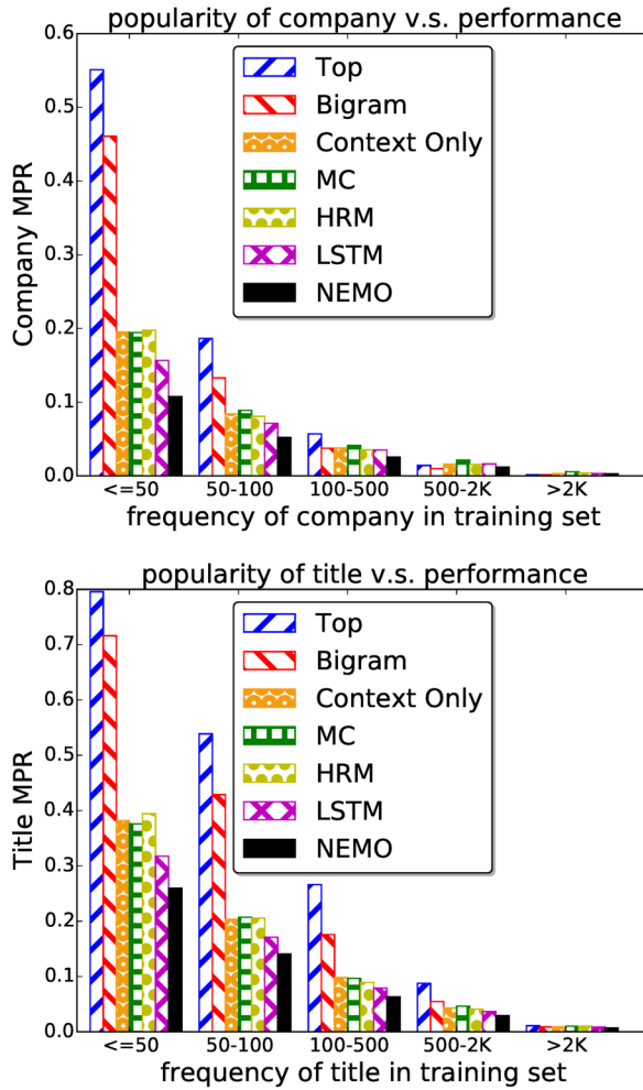
Figure 4: Performance with varying popularity of target company/title in Computer . The lower the better. Top: evaluation on company prediction. Bottom: evaluation on title prediction.
