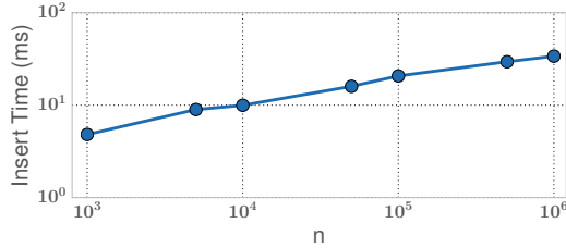
Figure 9: Per item insertion time for 100 items increases as n grows.
