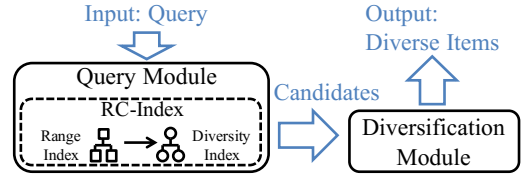
Figure 2: Solution overview. Our prototype system involves two modules: the Query Module and the Diversification Module.
