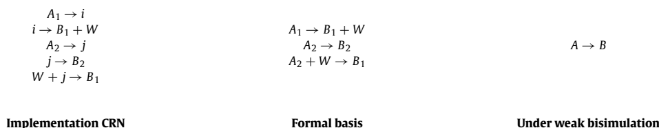
Fig. 4. The compositional hybrid approach for verifying an implementation of the formal CRN \{A \rightarrow B\} . We first apply pathway decomposition, treating the upper case species as formal species and lower case species as intermediate species. Then, we apply weak bisimulation using the natural interpretation which interprets A_1 and A_2 as \{A\} , B_1 and B_2 as \{B\} , and W as \emptyset . Thus, in two steps, the implementation CRN has been shown to be a correct implementation of \{A \rightarrow B\} .
