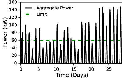
Figure 6: Aggregate power of the 18 homes over 30 days.
