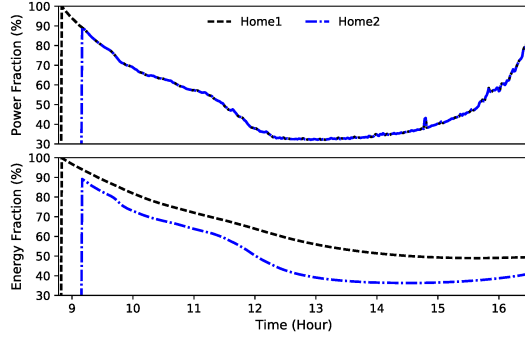
Figure 3: Divergence in the fraction of energy contributed by Homes 1 and 2 from Figure 2, even when the fraction of power they contribute is equal, assuming a 5kW limit.
