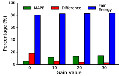
Figure 14: Impact of accelerating the “catch up” of sites that are behind in their fair energy allocation by a multiplicative gain factor in the distributed algorithm.
