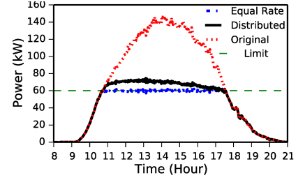
Figure 13: Maintaining the limit at a 1-minute interval.
