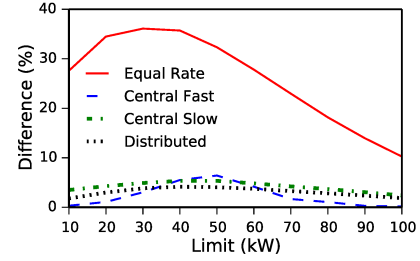
Figure 9: Energy difference between H1 and H18 in Figure 5(a), as a function of the aggregate limit.
