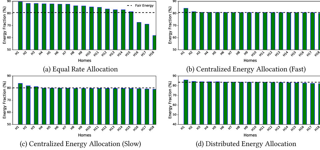
Figure 5: Distribution of energy allocation (relative to maximum energy potential) under a limit of 60kW for the equal rate (a), centralized fair energy (fast) (b), centralized fair energy (slow) (c), and distributed fair energy algorithms (d).
