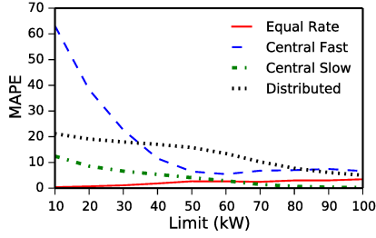
Figure 10: Fidelity of maintaining the aggregate limit as a function of its magnitude for the different variants.
