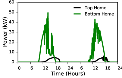
Figure 7: Daily profiles of home H1 and H18 in Figure 5(a).
