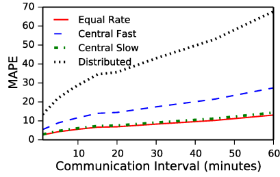
Figure 11: As the propagation delay increases the fidelity of control for the distributed algorithm decreases.
