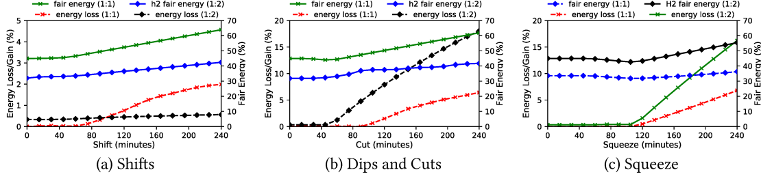
Figure 4: Impact on energy fairness as a function of the magnitude of shifts (a), cuts (b), and squeezes (c) for two solar sites.
