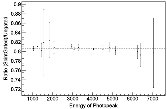
FIG. 5. Ratio of the measured photopeak integral in the scintillator-gated \gamma -ray spectrum to the measured integral in the ungated spectrum, the mean of the measurements (black dashed line, 80.6%) and the one-sigma envelope denoting the standard deviation of the points about that mean (dashed lines, 0.7%).
