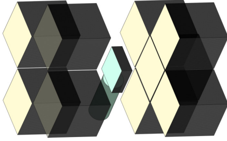
FIG. 3. Simple schematic showing the relative positions of the central scintillator and the surrounding germanium clover detectors (solid angle 6.8 sr). The ^{31}\text{Cl} beam particles are implanted from the left into central scintillator, which detects the \beta particles. The subsequent \gamma rays emitted by the daughter ^{31}\text{S} nucleus are detected by the surrounding clover array.
