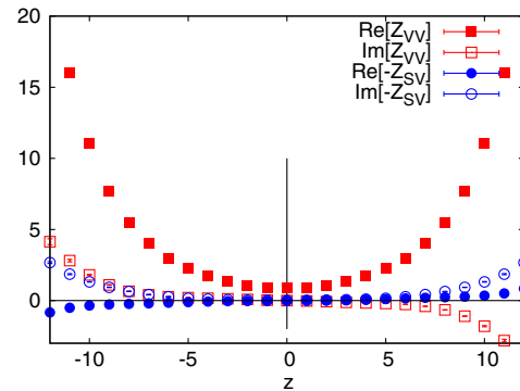
FIG. 2. The renormalization constant of the quasi-PDF operator O_{\gamma_z}(z) (red boxes) and the mixing with the scalar quasi-PDF operator O_I(z) (blue dots) with the momentum along the Wilson link being 6\pi/L = 1.29 \text{ GeV} and \mu_R^2 = p^2 = 5.74 \text{ GeV}^2 . The size of the mixing coefficient is about an order of magnitude smaller than the renormalization factor in the large- z region.
