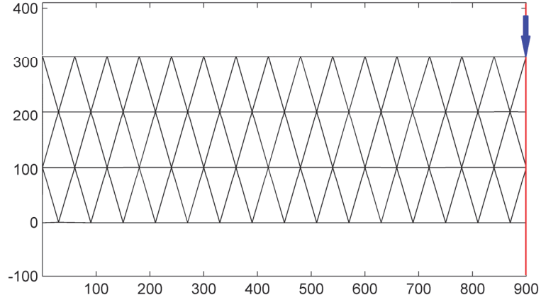
(a) Input base structure and the boundary condition
