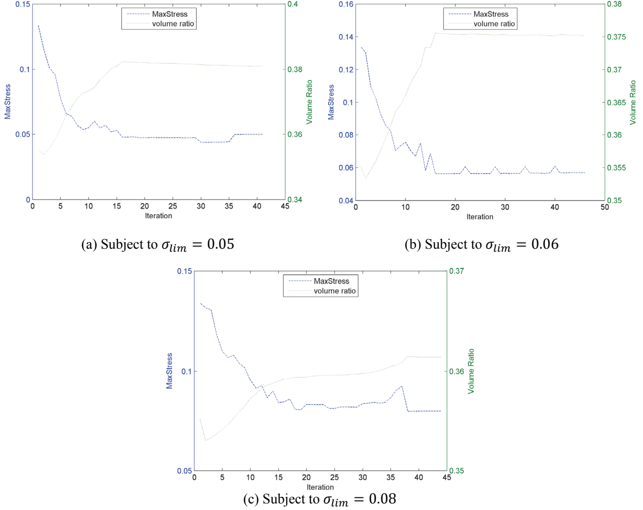
Figure 12. Convergence histories
