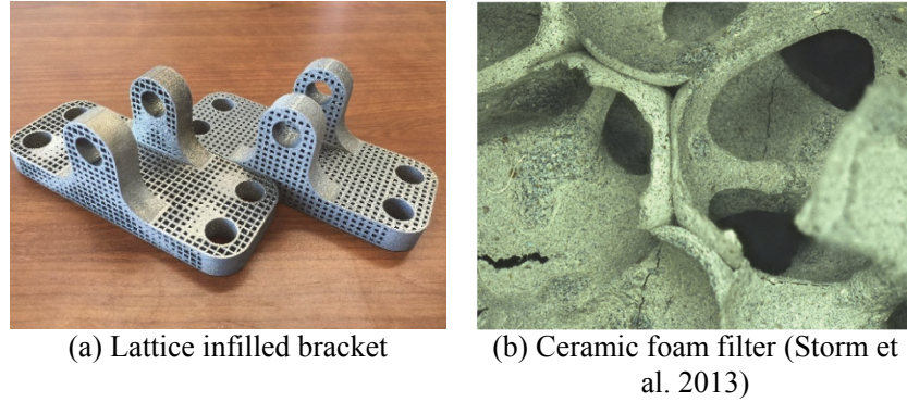
Figure 1. Examples of engineered porous structures
