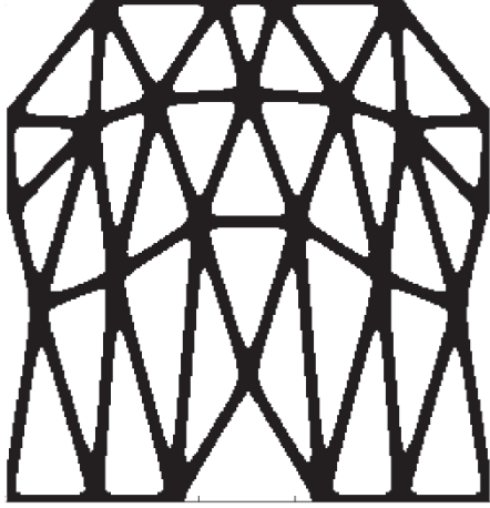
(c) Restored continuum structure
