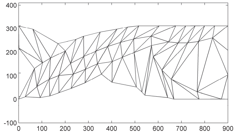
(b) Optimization result subjected to the \underline{S} = 1440
