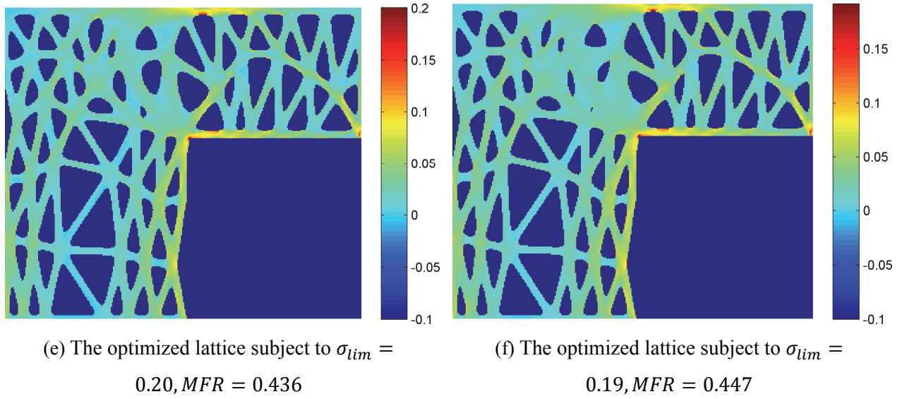
Figure 13. Trial solution on the L-bracket problem
