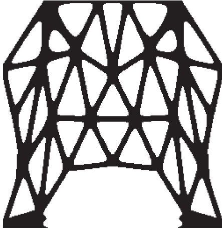
(a) The optimized lattice subject to \sigma_{lim} = 0.06, MFR = 0.366
