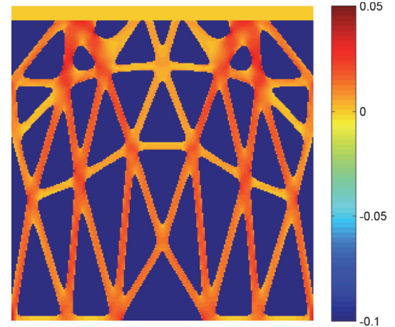
(b) The stress distribution
