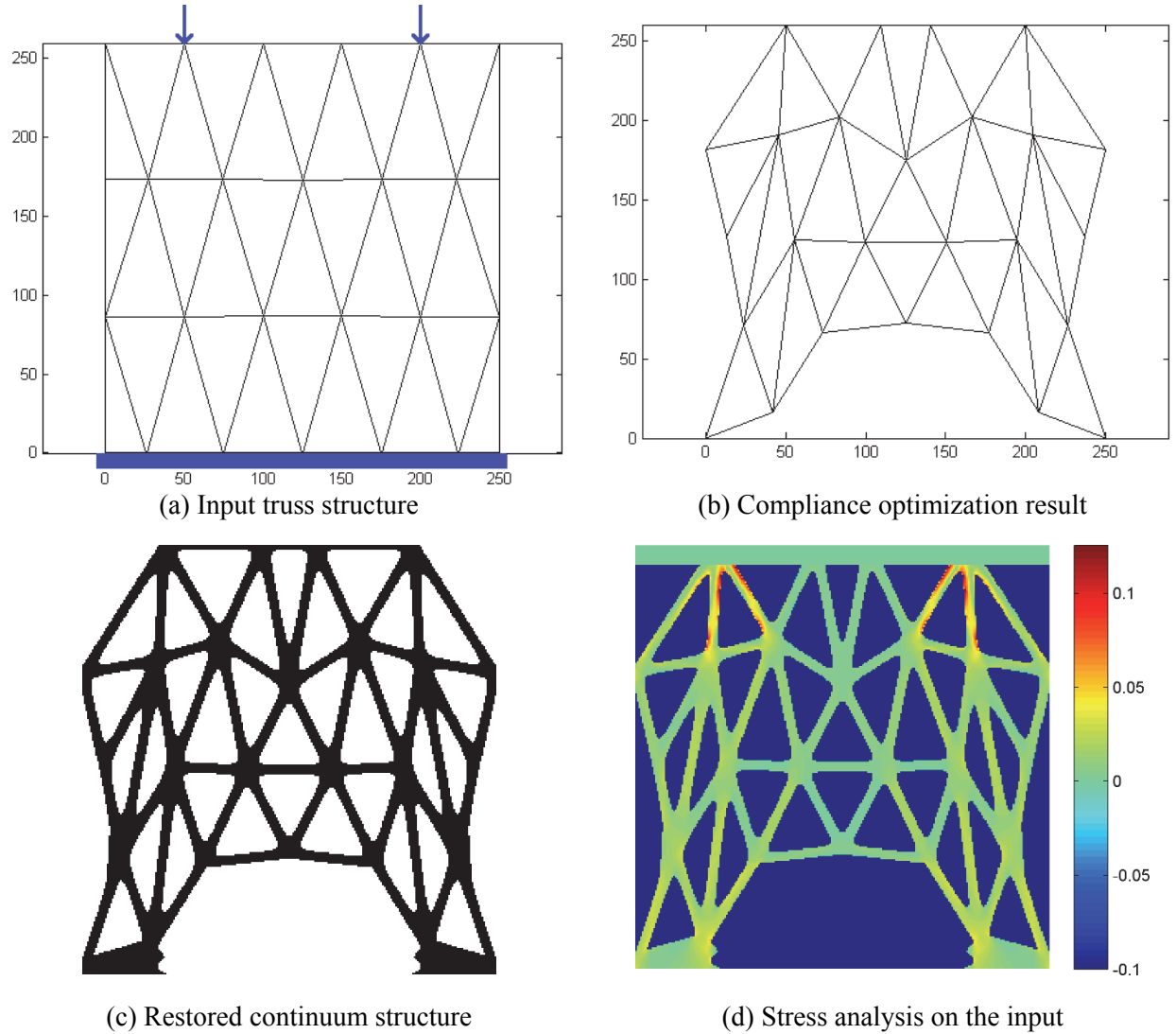
Figure 7. Truss structure optimization and the lattice transformation
