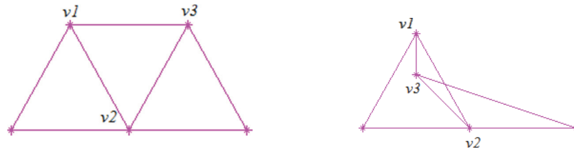
Figure 3. Example of truss element intersection: (a) Structure before truss element intersection, (b) Structure after truss element intersection.
