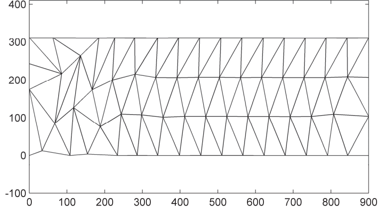
(d) Optimization result subjected to the \underline{S} = 2880
