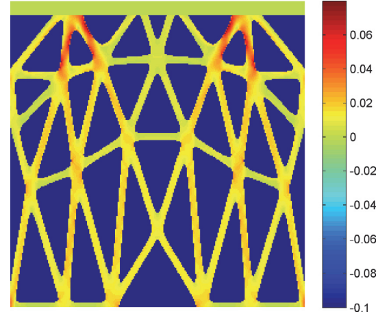
(f) The stress distribution
