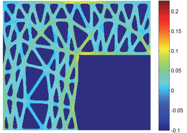
(d) Stress analysis on (c): maximum stress is 0.23 and the MFR is 0.409
