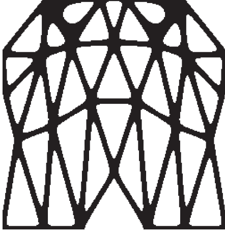
(c) The optimized lattice subject to \sigma_{lim} = 0.06, MFR = 0.375
