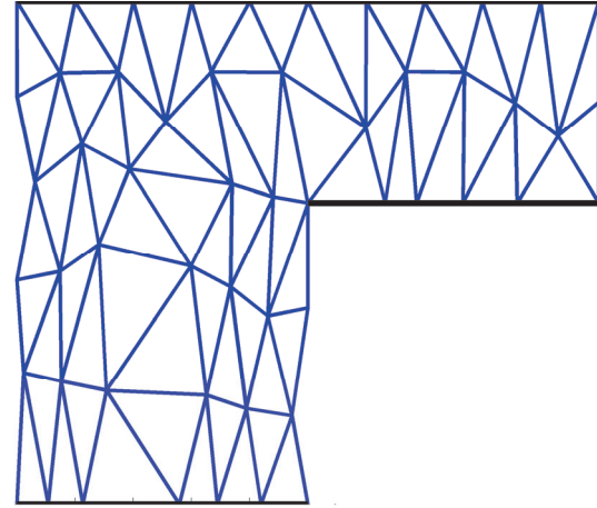
(b) Compliance minimization result
