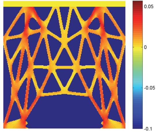
(b) The stress distribution
