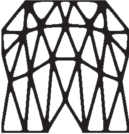
(e) The optimized lattice subject to \sigma_{lim} = 0.08, MFR = 0.361
