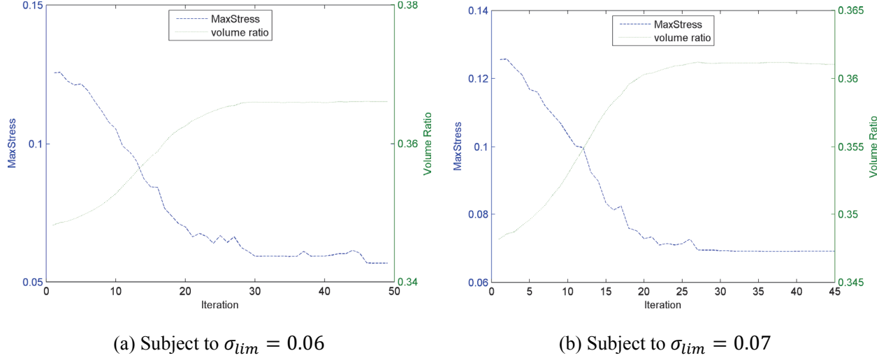
Figure 9. Convergence histories
