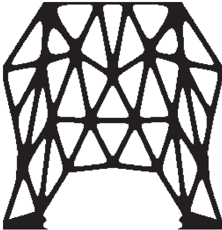
(c) The optimized lattice subject to \sigma_{lim} = 0.07, MFR = 0.361
