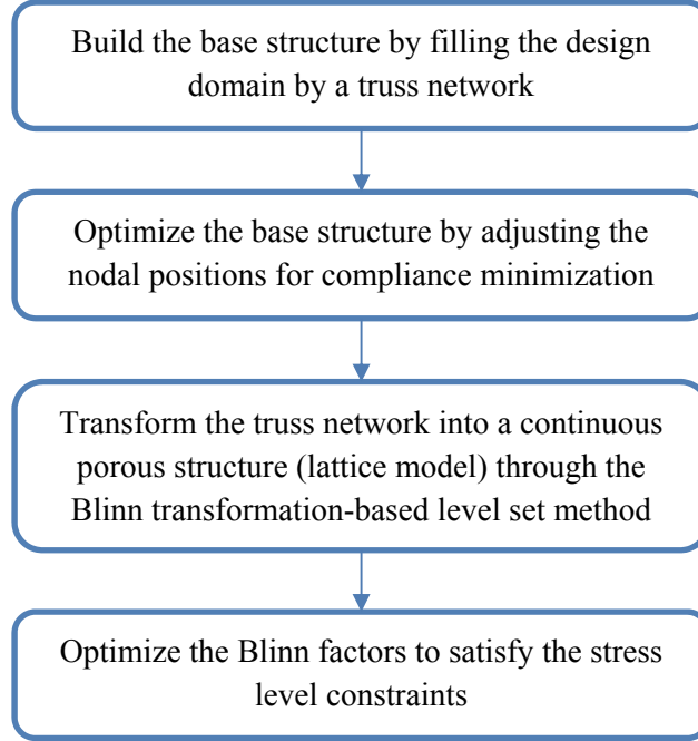
Figure 2. Overview of the proposed method
