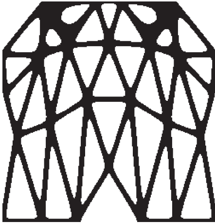
(a) The optimized lattice subject to \sigma_{lim} = 0.05, MFR = 0.381
