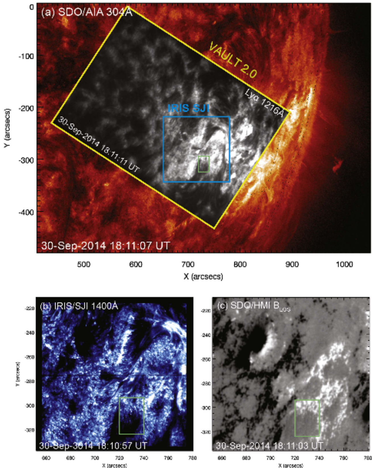
Figure 1. (a) Context image from AIA/SDO at 304 Å, showing the FOV of VAULT2.0 and IRIS. The green box shows a region of 20'' \times 30'' centered at the location of the Type-II spicule co-observed by VAULT2.0 and IRIS. (b) The FOV of IRIS SJI in 1400 Å. (c) The line-of-sight magnetogram from HMI/SDO for the FOV of panel (b) saturated at \pm 500 G. Light (dark) tones of gray correspond to positive (negative) magnetic polarities. The location where the type-II spicule and network jet occur (green box) is adjacent to a positive polarity plage region.
