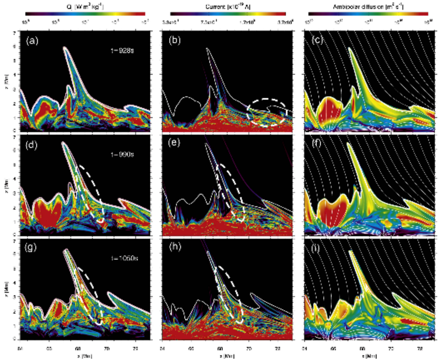
Figure 5. Joule heating, Q , the magnitude of electrical current, |J| , and ambipolar diffusion for the Type-II spicule of Figure 4 arranged in columns at three time instances of the simulation (rows at t = 928 , 990 , and 1050 s). The thick white (all panels) and pink (left) lines show T = 10^4 K and T = 10^5 K isocountours, respectively. Selected magnetic field lines are shown in the right panels (thin white lines). Note the evolution of ambipolar diffusion and the electrical currents with the receding temperature isocountour over time. At t = 928 s, electric currents between x = 71\text{--}73 Mm intensify (panel (b); white dashed oval) and at t = 990 s extend radially outward along the spicule (dashed oval in panel (c)), increasing the Joule heating and subsequently the temperature of the outer part of the spicule (dashed ovals in panels (d) and (g)).
