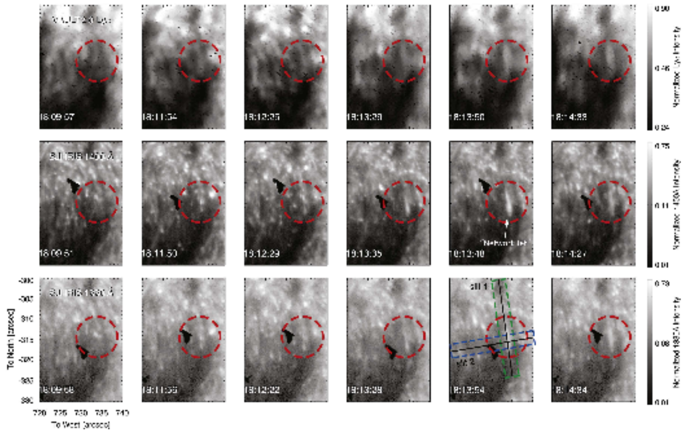
Figure 2. Time-evolution of a network jet observed in Ly \alpha 1216 Å by VAULT2.0 (top row) and with the IRIS slit-jaw imager in Si IV 1400 Å (middle row) and C II 1330 Å (bottom row). The FOV corresponds to the green box of Figure 1. Intensities for each passband I are normalized as I/I_{\max} with I_{\max} being the strongest intensity in the FOV of the entire time series. Scaling is logarithmic (base 10) for all panels. The sharp dark features in the IRIS FOVs are particles on the slit-jaw detector. The network jet occurs at the time shown in the last columns of Si IV 1400 Å and C II 1330 Å. The Ly \alpha counterpart of the network jet is shown inside the red dashed circle in the top row and it seems to pre-exist (at least in the panel at 18:11:54 UT) the appearance of the network jet (compare the content in red dashed circles between wavelengths). The green dashed rectangle shown in panel 18:13:54 marks the area containing the network jet and the blue dashed rectangle marks the area intersecting the network jet at approximately a 90° angle. Pixels along the dark lines inside these locations are used in the space-time plots of Figure 3.
