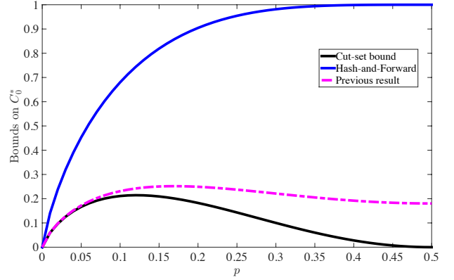
Fig. 2. Bounds on C_0^* .
