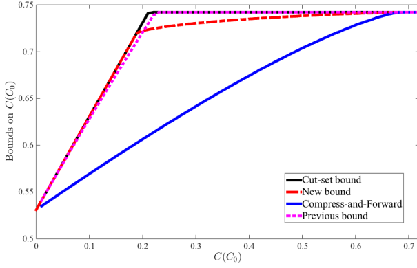
Fig. 3. Bounds on C(C_0) .
