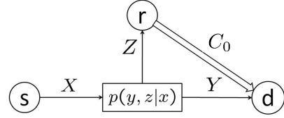
Fig. 1. A relay channel.
