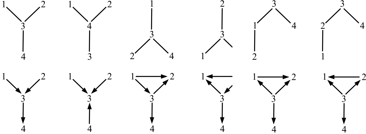
FIGURE 8. Posets and their corresponding DAGs representing the new (compared to the permutohedron) vertices of the DAG associahedron discussed in Examples 3.4 and 8.2.
