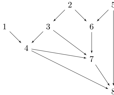
FIGURE 5. In the DAG, \bar{1} \rightarrow \underline{4} \leftarrow \overline{3} \leftarrow \overline{2} \rightarrow \underline{6} \rightarrow \underline{7} \leftarrow \overline{6} \leftarrow \overline{5} \rightarrow \underline{8} is a Bayes ball path from 1 to 8 given \{4, 7\} . The treks and canyons along the path are overlined and underlined respectively.
