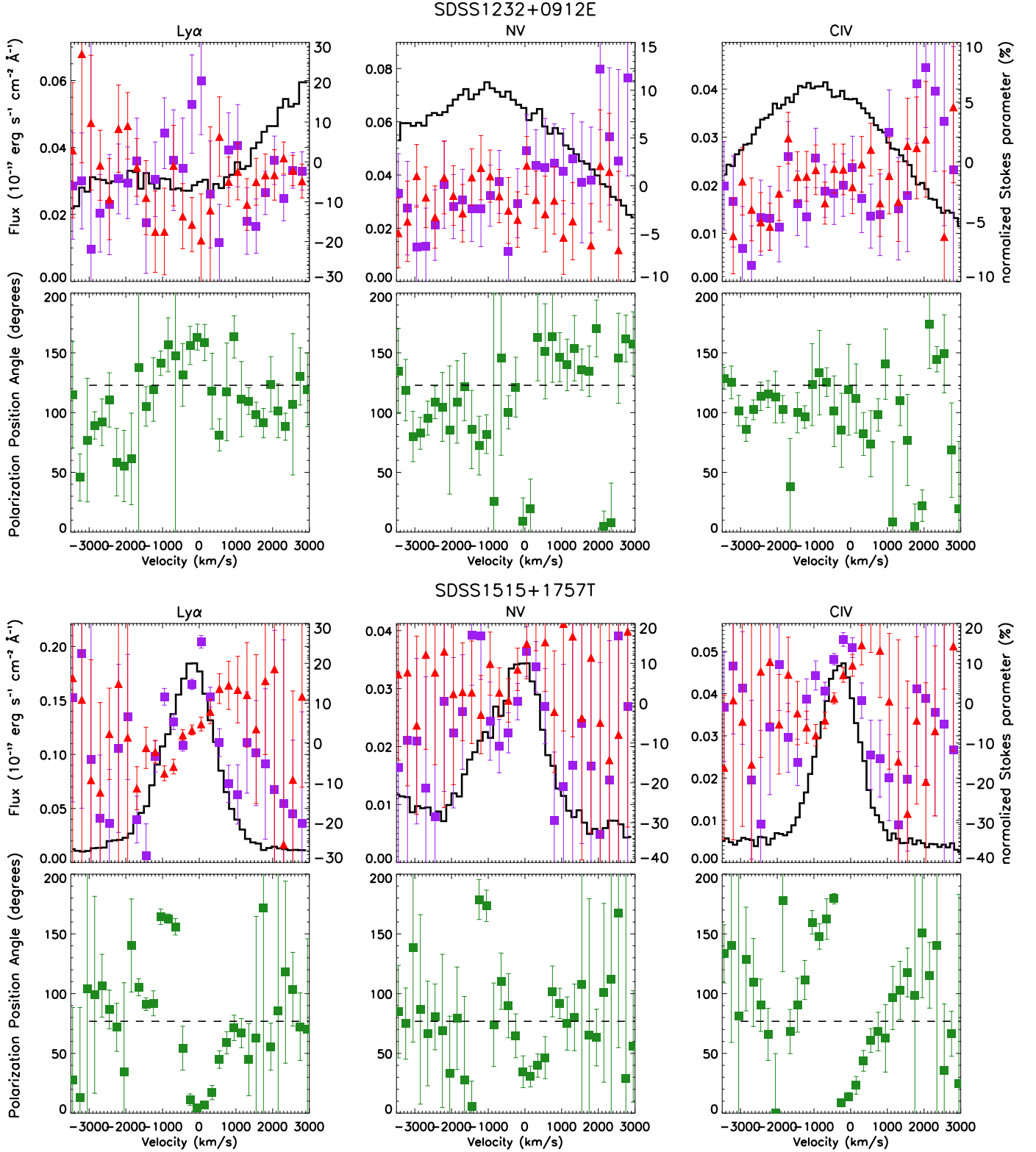
Figure A5. Emission line spectra of remaining targets (see Figure 3).
