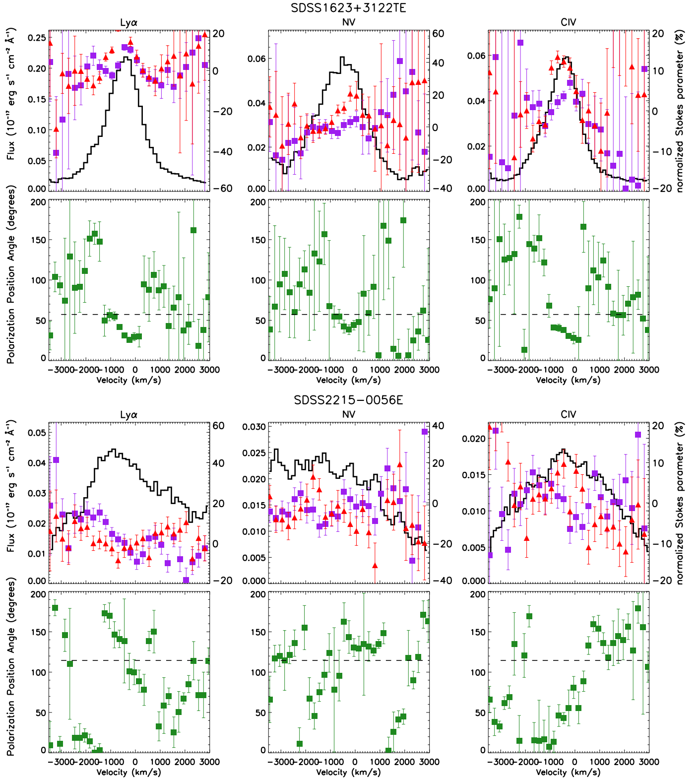
Figure A6. continued
