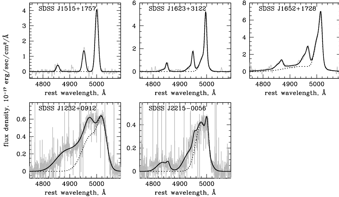
Figure 1. The continuum-subtracted [O III]+H \beta complex and best fits for the five objects studied in this paper. The spectra were obtained for the top three objects with Gemini GNIRS and have not previously been published. Spectra for the bottom two objects were obtained with the VLT XShooter and were published in Zakamska et al. (2016) . The grey histograms show the data, the solid black line shows the best overall fit and the dotted black line shows the [O III] \lambda 5007 Å fitted profile separately. In SDSSJ1515+1757T, SDSSJ1623+3122TE and SDSSJ1652+1728E the best fits are kinematically tied (i.e., [O III] and H \beta have the same velocity structure), and the best velocity fit is comprised of one, two and three Gaussian components, respectively. The best fits for SDSSJ1232+0913E and SDSSJ2215-0056E were previously presented in Zakamska et al. (2016) and are reproduced here. In SDSSJ1232+0913E, the best fit is kinematically untied; in SDSSJ2215-0056E it is kinematically tied; in both cases, two Gaussian components are used for [O III].
