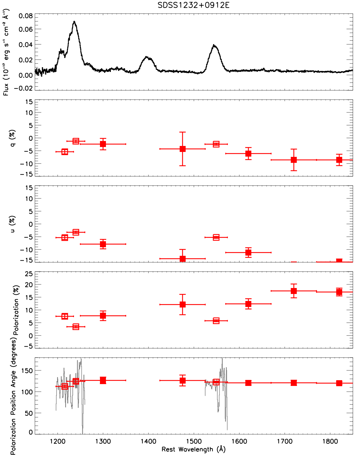
Figure A1. LRISp spectra of our remaining targets (see Figure 2).
