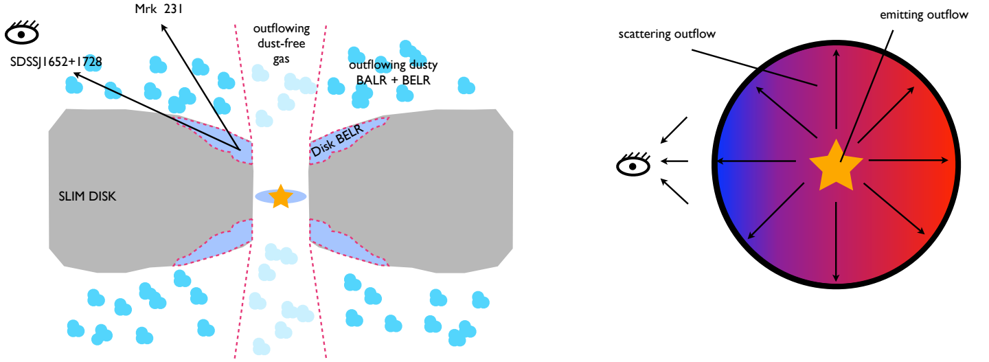
Figure 5. Our preferred model for SDSSJ1652+1728 is adapted from Veilleux et al. (2016). It combines a polar outflow which produces the emission lines with a dusty equatorial wind where the scattering occurs. Left: Side-on view of the inner \sim 10 pc of our model (not to scale). The inner accretion disk ( \lesssim 0.01 pc) is responsible for the X-ray emission and is surrounded by a geometrically-thick accretion disk (“slim disk”) which, for a near- or super-Eddington quasar produces narrow funnels that drive a polar wind. This polar wind is comprised of both dust-free outflowing gas, responsible for X-ray absorption, as well as dusty clouds that produce FeLoBAL absorption signatures and the blueshifted FUV emission lines of Ly \alpha and C IV. The extended accretion disk is the source of the UV and optical continuum emission as well as the Balmer lines (seen through the screen of the outflowing dusty BALR). Mrk 231 is constrained to have a jet angle of \theta_{max} = 25.6^{+3.2}_{-2.2} degrees from radio observations (Reynolds et al. 2013). This means that the scattered light, though still significant, is unpolarized in the observer’s line of sight due to geometric cancellation. In contrast, SDSSJ1652+1728 is seen at a larger angle to the jet or polar axis as inferred from the mean SED of ERQs (see section 4.1 for further discussion). The increased column density of obscuration suppresses the FeLoBAL features while the more edge-on sight line reduces geometric cancellation of the polarization signature. Though the original cartoon from Veilleux et al. (2016) contains a radio jet we omit this as it is not the subject of this work. Right: The same model as viewed from above (looking along the polar axis). Here we show how the kinematic features in the polarized emission-line regions are created by the blue and red-shifted scattering emission respectively. The viewer (eye on the left) sees blueshifted emission coming towards them and scattered off of clouds moving towards the observer. In contrast, the redshifted wings of the emission lines are dominated by scattering off the “sides” of the outflow (from the observer’s perspective). Emission from the back of the cone is largely suppressed in polarization because the scattering efficiency is low at angles \gtrsim 90 degrees, though this emission does contribute to the overall redshift of polarized emission lines compared to the unpolarized emission lines. These features combined produce the ninety degree rotation in the polarization position angle across the emission lines.
