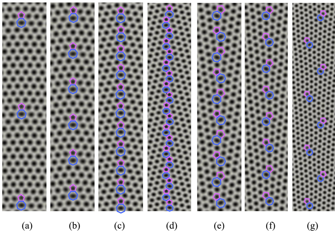
Fig. 3. Density fields predicted by the PFC model for GBs with misorientation angles of: (a) \theta = 5.09 , (b) \theta = 13.17 , (c) \theta = 21.79 , (d) \theta = 32.2 , (e) \theta = 42.1 , (f) \theta = 46.83 , and (g) \theta = 50.57 .
