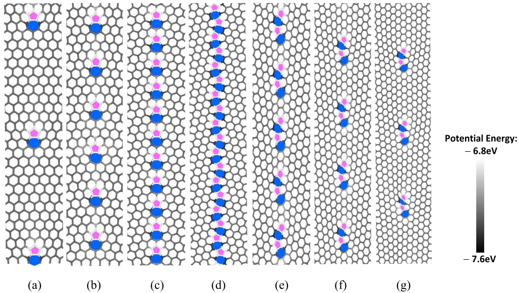
Fig. 1. Atomic structures of GBs constructed from CSL with misorientation angles of: (a) \theta = 5.09 , (b) \theta = 13.17 , (c) \theta = 21.79 , (d) \theta = 32.2 , (e) \theta = 42.1 , (f) \theta = 46.83 , and (g) \theta = 50.57 .
