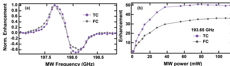
Fig. 6 Normalized DNP profiles comparing the freezing conditions (FC and TC) of 5 mM 4AT in 5 : 4 : 1 (a) and the power curves of the same sample obtained at 193.65 GHz of MW irradiation (b) at 4 K and 6.95 T. The DNP profiles were normalized to the maximum of the signal intensity and the frequency was scaled by 4 GHz to represent data acquired at 7 T for comparison to the rest of the data presented here. Lines are drawn to guide the eye.
