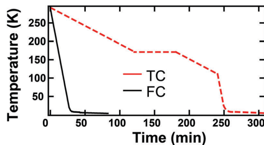
Fig. 1 Time versus temperature depiction of the two freezing conditions: fast cool (FC) 10\text{ K min}^{-1} from 290 K to 4 K [black – solid] and thermally controlled (TC) 1\text{ K min}^{-1} from 290 K to 10 K above T_g , then 1\text{ K min}^{-1} to 100 K followed by 12\text{ K min}^{-1} to 4 K [red – dashed]. Temperature was monitored with a Lake Shore Cernox ® temperature sensor.
