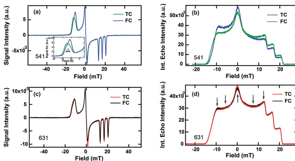
Fig. 3 EPR lineshapes of 40 mM 4AT in 5:4:1 (a and b) and 6:3:1 (c and d) d_8 -glycerol: D_2O : H_2O at 8.56 T and 4.5 K. cw-EPR (a and c) and field swept echoes (b and d) are shown for both freezing conditions: fast cool (FC) and thermally controlled (TC). The inset in (a) shows the shift in g_{xx} annotated by \Delta , corresponding to 250 ppm, where g_{xx} shifts from 2.00839 to 2.00787. All spectra have been normalized to the double integral. The arrows in (d) are to show the relative position of the T_m measurements in Fig. 3.
