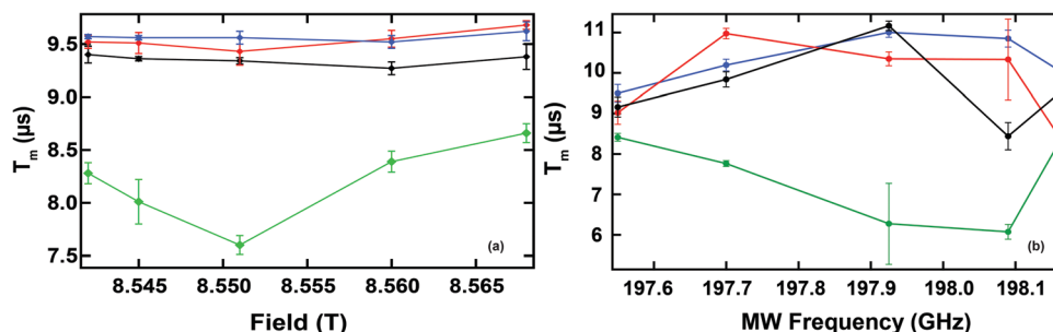
Fig. 4 T_m was plotted as a function of the relative position along the EPR line as indicated in Fig. 2d for the different freezing conditions and model solutions of 40 mM 4AT as defined by the color code inside the plot, where (a) indicates T_m measured at 4.5 K and at 8.56 T (240 GHz) and (b) indicates T_m measured at 4 K and at 7 T (198 GHz). Lines are drawn to guide the eye.
