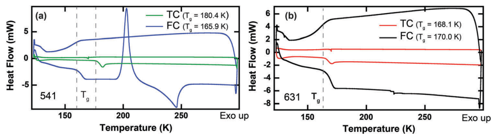
Fig. 2 DSC plots of the different freezing conditions fast cool (FC) and thermally controlled (TC) for 40 mM 4AT in 5:4:1 (a) and 6:3:1 (b) d_8 -glycerol: D_2O : H_2O . The T_g from each of the heating curves are noted in the plots by dashed grey vertical lines. The cooling curves are the top curves, while the heating curves are the bottom curves. Exothermic events are on top.
