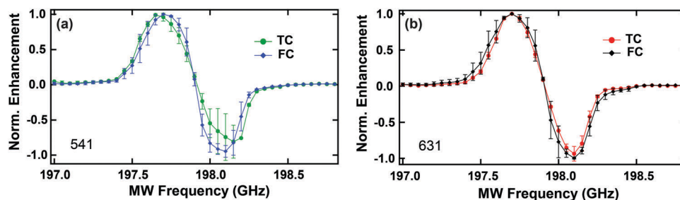
Fig. 5 Normalized average DNP profiles comparing the freezing conditions (FC and TC) of 40 mM 4AT in 5 : 4 : 1 (a) and 6 : 3 : 1 (b) \text{d}_8 -glycerol : \text{D}_2\text{O} : \text{H}_2\text{O} taken at 7 T and 4 K. All spectra were normalized to the maximum signal intensity and standard deviations are shown to indicate the variability from day-to-day for the triplicated data sets. Lines are drawn to guide the eye.
