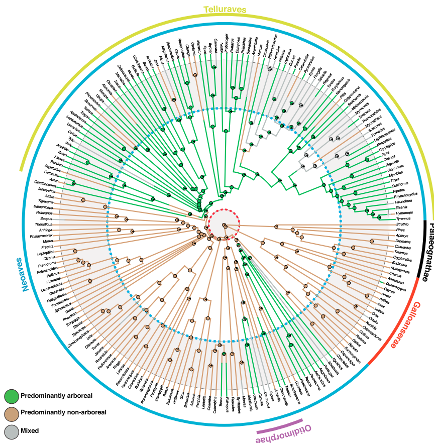
Figure 1. Ancestral Ecological Reconstructions Reveal Bias toward Non-arboreal Birds across the K-Pg
