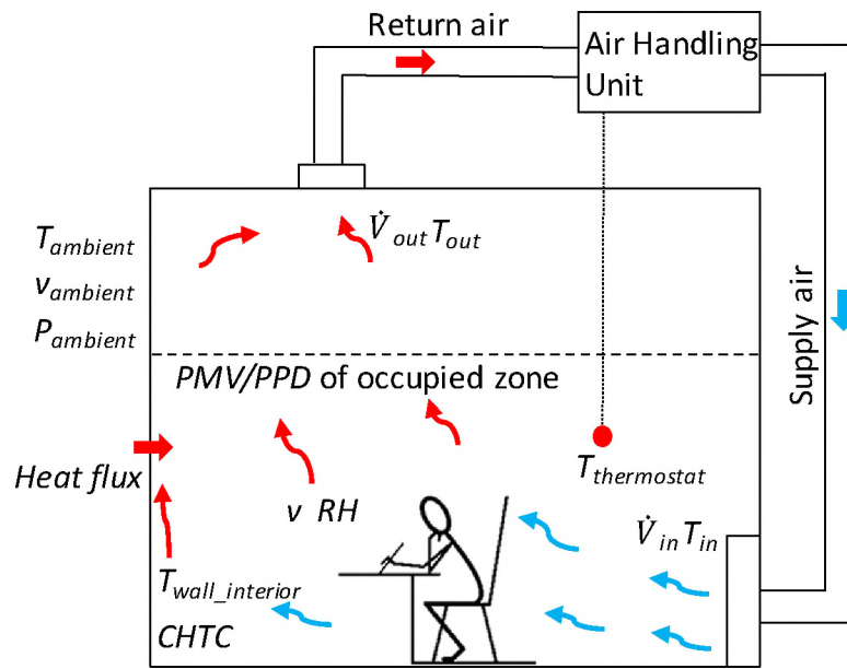
Figure 1 Exchanged data in a displacement ventilation system
