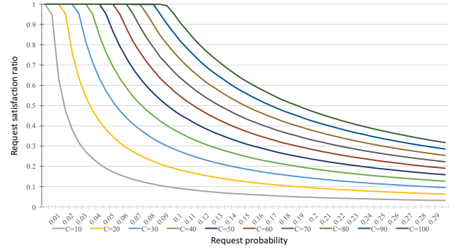
Figure 3. Request satisfaction-ratio of different grid loads.
