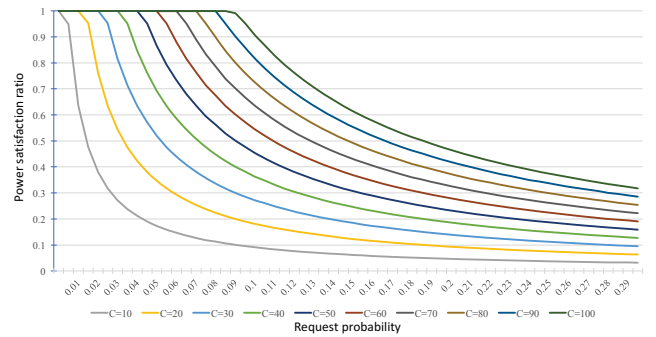
Figure 4. Power satisfaction ratio of different grid loads.
