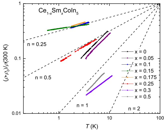
FIG. 13. Plot of \log[(\rho - \rho_0)/\rho(300 \text{ K})] vs \log T for \text{Ce}_{1-x}\text{Sm}_x\text{CoIn}_5 ( 0 \leq x \leq 0.5 ) up to T \approx 15 \text{ K} . Linear behavior indicates power-law behavior given by Eq. (5). Dashed lines are provided at exponents of n = 0.5, 1 , and 2 as guides to the eye.
