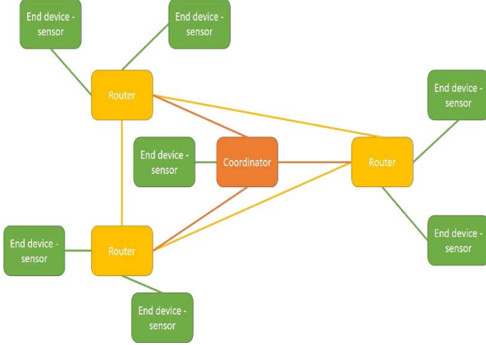
Figure 4. Example of a Mesh topology.
