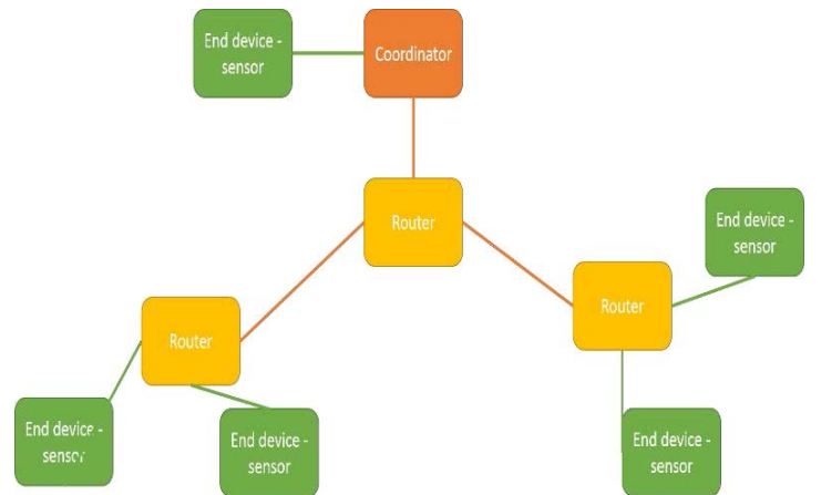
Figure 3. Example of a tree topology.
