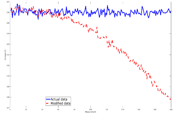
Figure 10. Voltage evolution (real - blue, transmitted - red)
