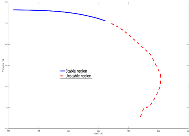
Figure 7. Stability region of the P - |V| curve
