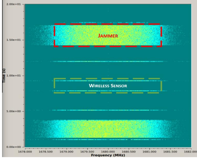
Figure 9. Spectrum waterfall plot for jammer experiment
