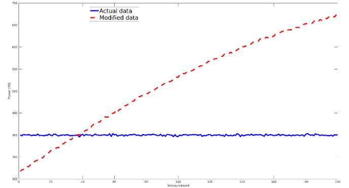
Figure 11. Power evolution (real - blue, transmitted - red)
