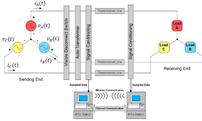
Figure 1: 3-Phase Power System
