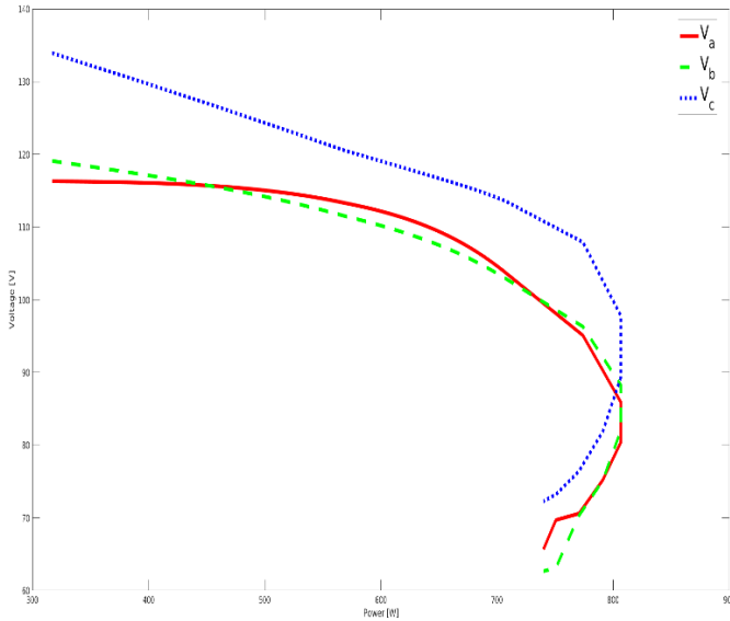
Figure 2. Power - Voltage curve for all phases.
