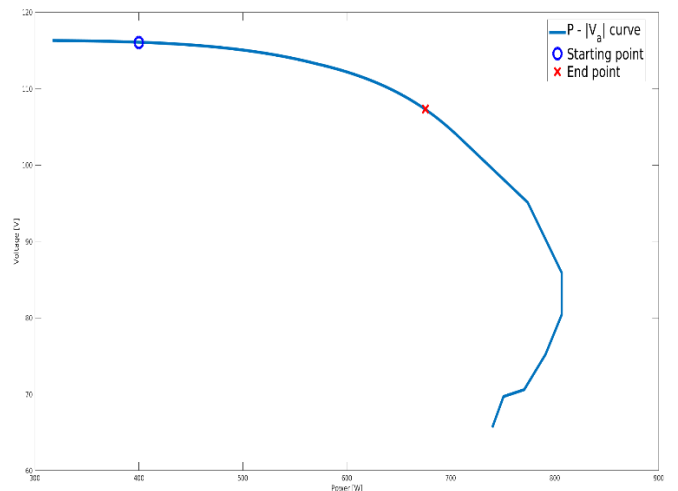
Figure 12. Received P - |V| curve for one phase.
