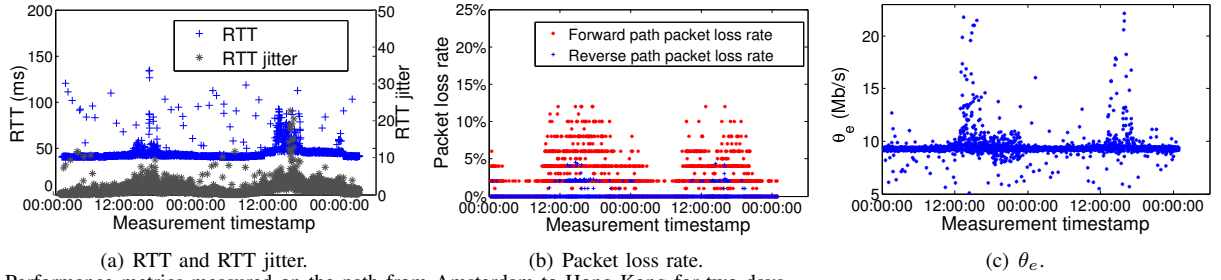
Fig. 19. Performance metrics measured on the path from Amsterdam to Hong Kong for two days.
