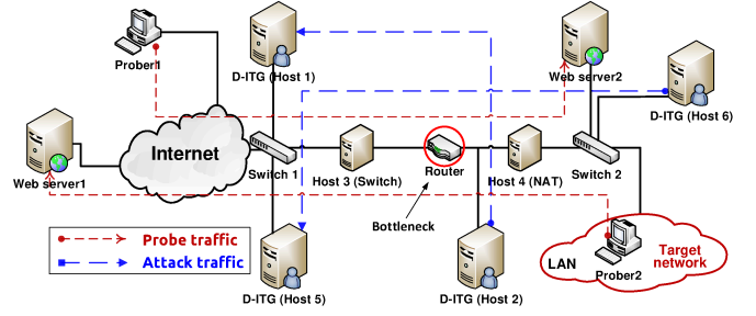
Fig. 11. The topology of the testbed.
