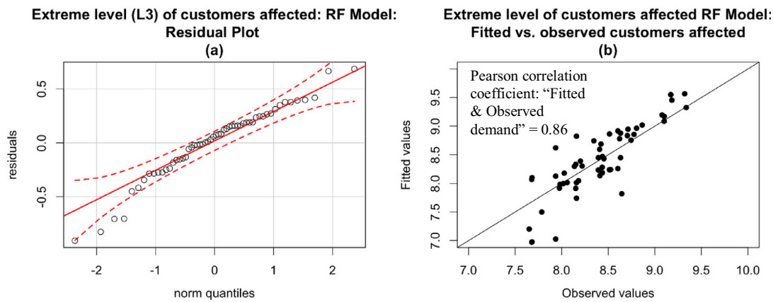
Fig. 14. Extreme level of customers affected RF Model: (a) QQ-plot (the red dashed lines in the QQ-plot represent 95% confidence intervals) and (b) Fitted values vs. observed values. (For interpretation of the color code in this figure legend, the reader is referred to the web version of this article.)
