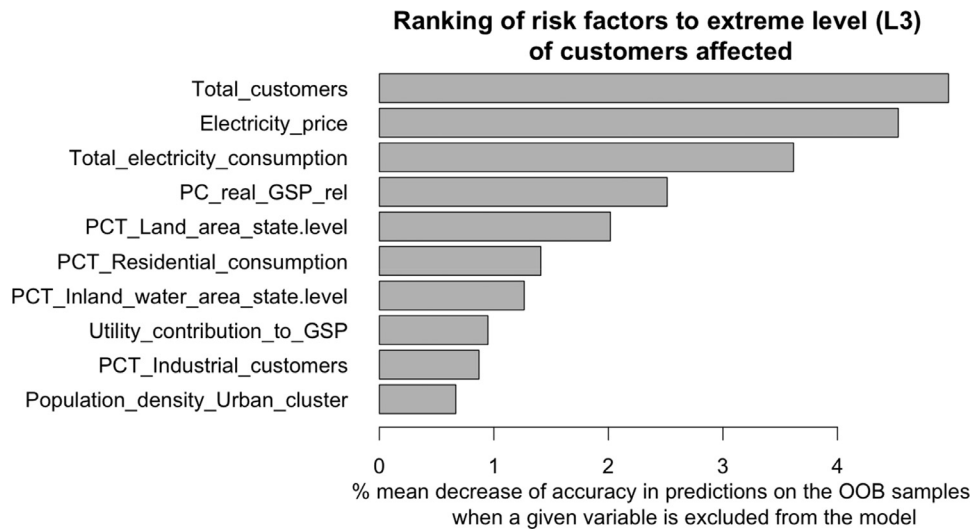
Fig. 16. Ranking of the risk factors contributing to higher number of customers affected.
