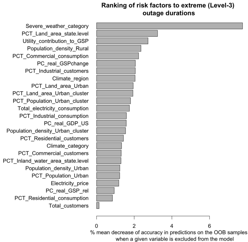
Fig. 15. Ranking of the risk factors contributing to prolonged outage duration.
