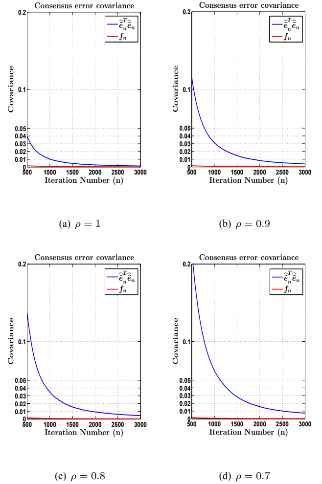
Fig. 8. Evolution of the theoretical asymptotic covariance f_n = \text{Trace}(\bar{M}_0^{-1} \Sigma_0 (\bar{M}_0^{-1})') and the empirical one obtained by simulation \hat{\bar{e}}_n^T \hat{\bar{e}}_n under Markovian communication erasure channels.
