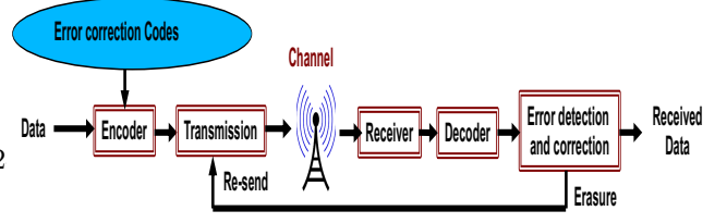
Fig. 1. An erasure channel with error detection and correction and re-transmission
