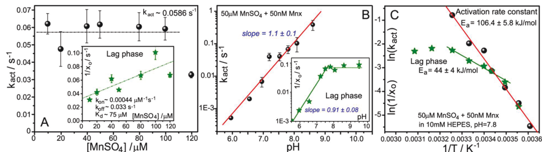
Figure 4. Dependence of the lag phase and activation rate constant parameters on (A) starting \text{MnSO}_4 concentration (in HEPES, pH 7.8), (B) pH (various buffers, 50 \mu\text{M} \text{MnSO}_4 starting concentration), and (C) temperature (50 \mu\text{M} \text{MnSO}_4 starting concentration, in HEPES, pH 7.8). (A) The activation rate constant is independent of \text{MnSO}_4 concentration, while the lag rate increases linearly, consistent with slow and weak ( K_{\text{d}} = 75 \mu\text{M} ) binding; the green line is the fit to eq 4, r = 0.793 . (B) The log of the activation rate constant shows a unit-slope linear increase with pH (linear fit: r = 0.981 ), as does the lag rate, which, however levels off above pH 7.8 (linear fit: r = 0.988 ). (C) Arrhenius plots for the activation rate constant (black dots; linear fit: r = 0.993 ) and the lag rate (green stars; linear fit: r = 0.989 ).
