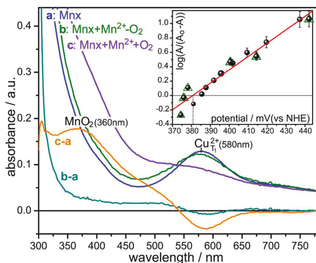
Figure 2. Absorption spectra of as-isolated Mnx protein (a, blue trace), and Mnx protein anaerobically incubated with 7 equiv of \text{Mn}^{2+}(\text{aq}) for ~1.5 h (b, green trace) and then mixed with \text{O}_2 -saturated buffer solution for 15 min (c, purple trace). Subtracting trace a from trace b shows a small background and a negligible 580 nm absorption loss (dark cyan trace). A substantial 580 nm absorption loss is seen (orange trace) against the \text{MnO}_2 background absorption (maximum at ~360 nm) when trace a is subtracted from trace c. The spectrum b has been scaled by the dilution factor. The inset shows the plot of eq 2 for the poised potential titration of Mnx (black points and green triangles) and the linear correlation (red line, r = 0.978 ) with the x -intercept giving the reduction potential of T1Cu as 380 \pm 5 mV (pH 7.8). The titration conditions were as follows: the black circles are starting with 0.5 mM \text{K}_3[\text{Fe}(\text{CN})_6] in pH 7.8 phosphate buffer and titrating with aliquots of 5 mM \text{K}_4[\text{Fe}(\text{CN})_6] ; the green triangles are starting with 0.5 mM \text{K}_3[\text{Fe}(\text{CN})_6] in pH 7.8 phosphate buffer and titrating with aliquots of 6 mM \text{K}_4[\text{Fe}(\text{CN})_6] .
