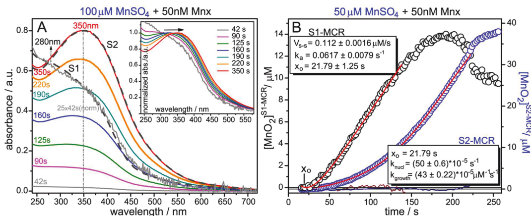
Figure 3. (A) UV-vis spectra taken at the indicated times during the Mn-catalyzed oxidation of 100 \mu\text{M} \text{MnSO}_4 in 10 mM HEPES buffer, pH 7.8. The product of the reaction, nanoparticulate \text{MnO}_2 , has a broad absorption band, which undergoes a red shift as it grows. The spectral profiles of the first (S1, black dashed line) and second (S2, black dashed line) components of the MCR-ALS multivariate analysis are superimposed on the normalized experimental spectra at 42 s (dark gray line) and 350 s (red line). Inset: The same UV-vis spectra on a normalized absorbance scale to show the red shift of the \text{MnO}_2 band more clearly. (B) Time profiles of the S1 (black points) and S2 (blue points) components obtained after the MCR-ALS procedure was applied to the data for 50 \mu\text{M} \text{MnSO}_4 and 50 nM Mn in 10 mM HEPES, pH 7.8. (Only the visible light source was used, to avoid UV photoreaction of HEPES, see Figure S2 in SI.) The red line on top of the S1 component is the fit to the activation equation (eq 3), ( r = 0.998 ), and the dark red line shows the residuals. The fitted time interval (up to 140 s) was selected before the slowing down of the steady-state rate due to substrate exhaustion. The red line on top of the S2 component is the fit to the agglomeration growth equation (eq 6) ( r = 0.9994 ), and the dark blue line is the residual for the fit.
