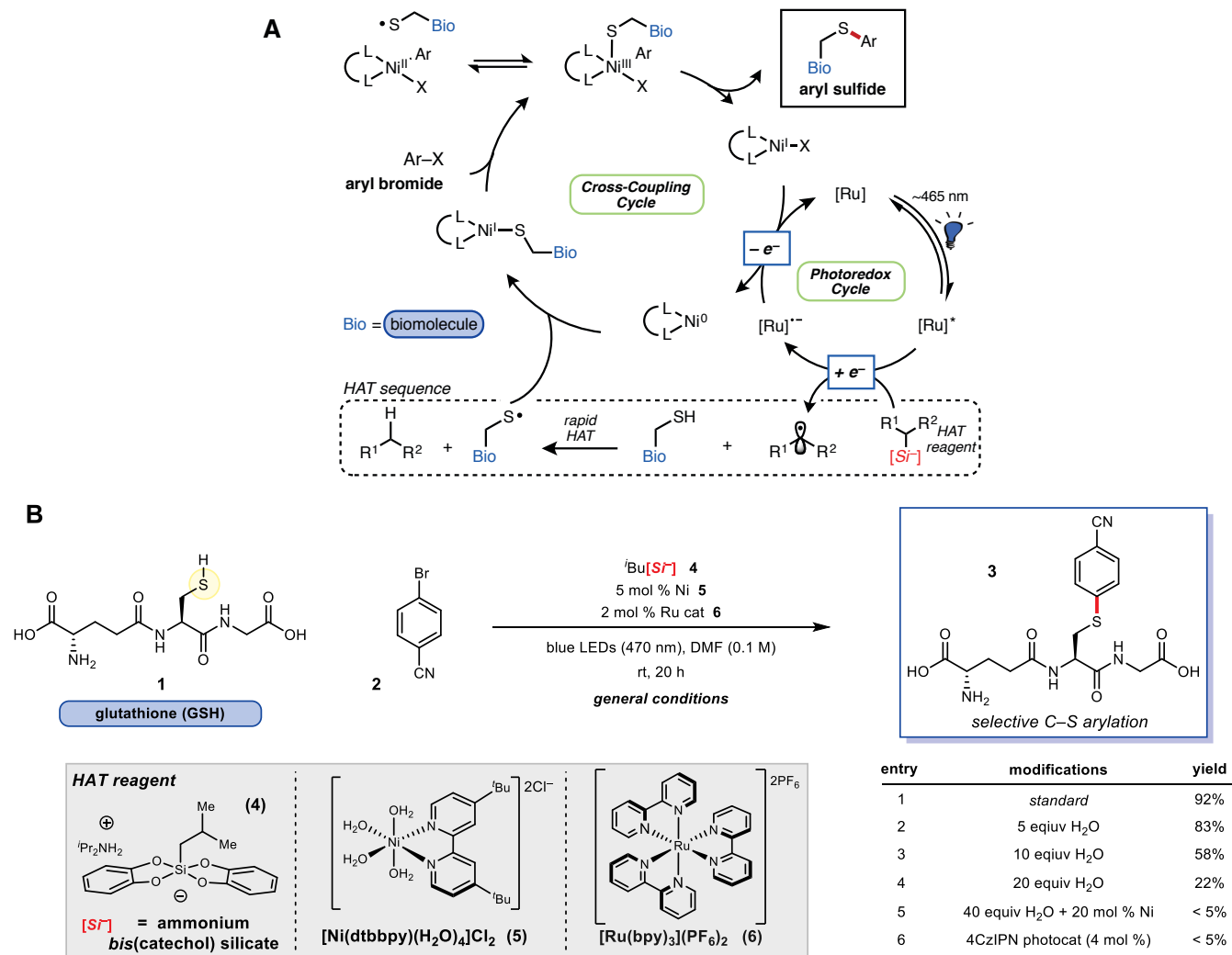
Figure 1. Proposed Ni/photoredox catalytic cycle and thioarylation reaction scheme. (A) Catalytic cycle is initiated by photon absorption, generating excited state Ru photocatalyst, followed by oxidation of the HAT reagent via SET. Rapid H-atom abstraction from the sulfhydryl group generates a thiyl radical, which adds to Ni(0). This is followed by Ni(I) oxidative addition 23 with the requisite aryl bromide. Reductive elimination from Ni(III) affords the desired thioarylated biomolecule, and the dual catalytic cycles are closed by a final SET. (B) Ni/photoredox thioarylation reaction with GSH (1) and 2 affords the arylated peptide. Select experiments are outlined that deviate from the general conditions. Additional experiments and the structure of 4CzIPN can be found in the Supporting Information.
