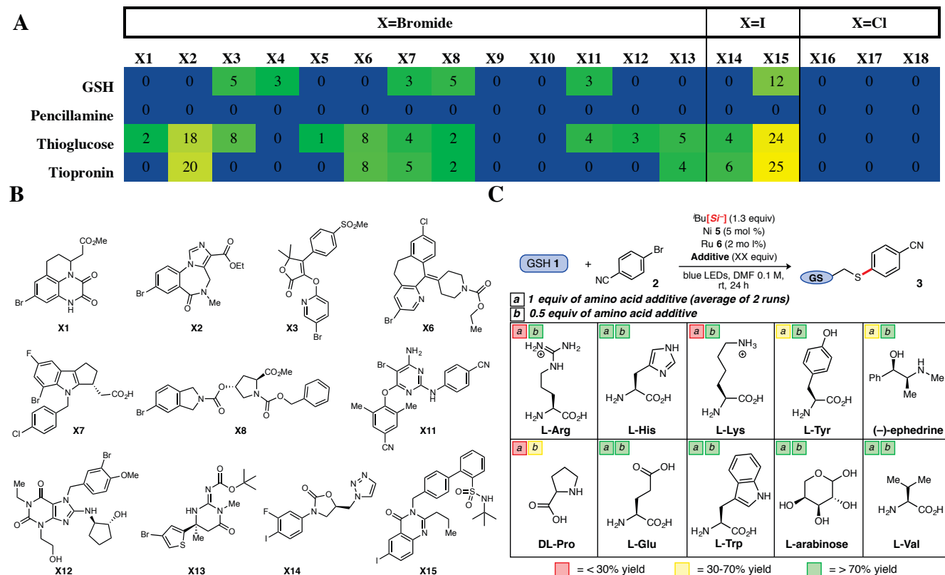
Figure 2. Rapid exploration of Merck aryl halide informer plate via HTE and tolerability studies of biological additives under optimized conditions. (a) Merck halides run with 4 diverse thiols; reported numbers in cells present product area%/internal std area% (normalized). (b) Structures of successful Merck halides ( X1 - X15 ) as explored in A. (c) Biological additives (1 equiv, box a; 0.5 equiv, box b) were screened under optimized conditions; yield determined vs. internal standard (average of 2 runs).
