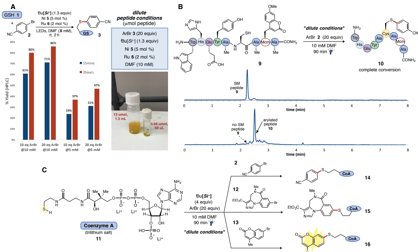
Figure 3. Application of thioarylation reaction conditions to native and diverse biological substrates. (a) Optimized “dilute conditions” with GSH at 10 mM for enabling small-scale peptide thioarylations. Employing 20 equiv of aryl bromide, 2 was found to increase relative reaction rate, as compared to 5 mM reactions vs. time. (b) Peptide 9 was subjected to optimized conditions at 10 mM for 90 min under blue LED irradiation. HPLC chromatogram depicts reaction progression and formation of product (see Supporting Information for reaction details). (c) Thioarylation of Coenzyme A ( 11 , 3Li salt) with three diverse aryl bromides (4 equiv silicate 4 employed) afforded the conjugated products under the developed conditions in all cases.
