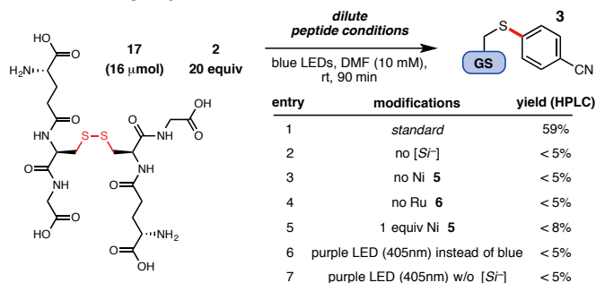
Figure 4. (a) Demonstration of reaction scalability for the Ni/photoredox thioarylation of peptides (see Supporting Information for details); isolated yields reported. (b) Dilute conditions employed: 5 mol % Ni 5 , 2 mol % Ru 6 , and 1.5 equiv silicate 4 . HPLC yields reported via product/internal standard ratios.
