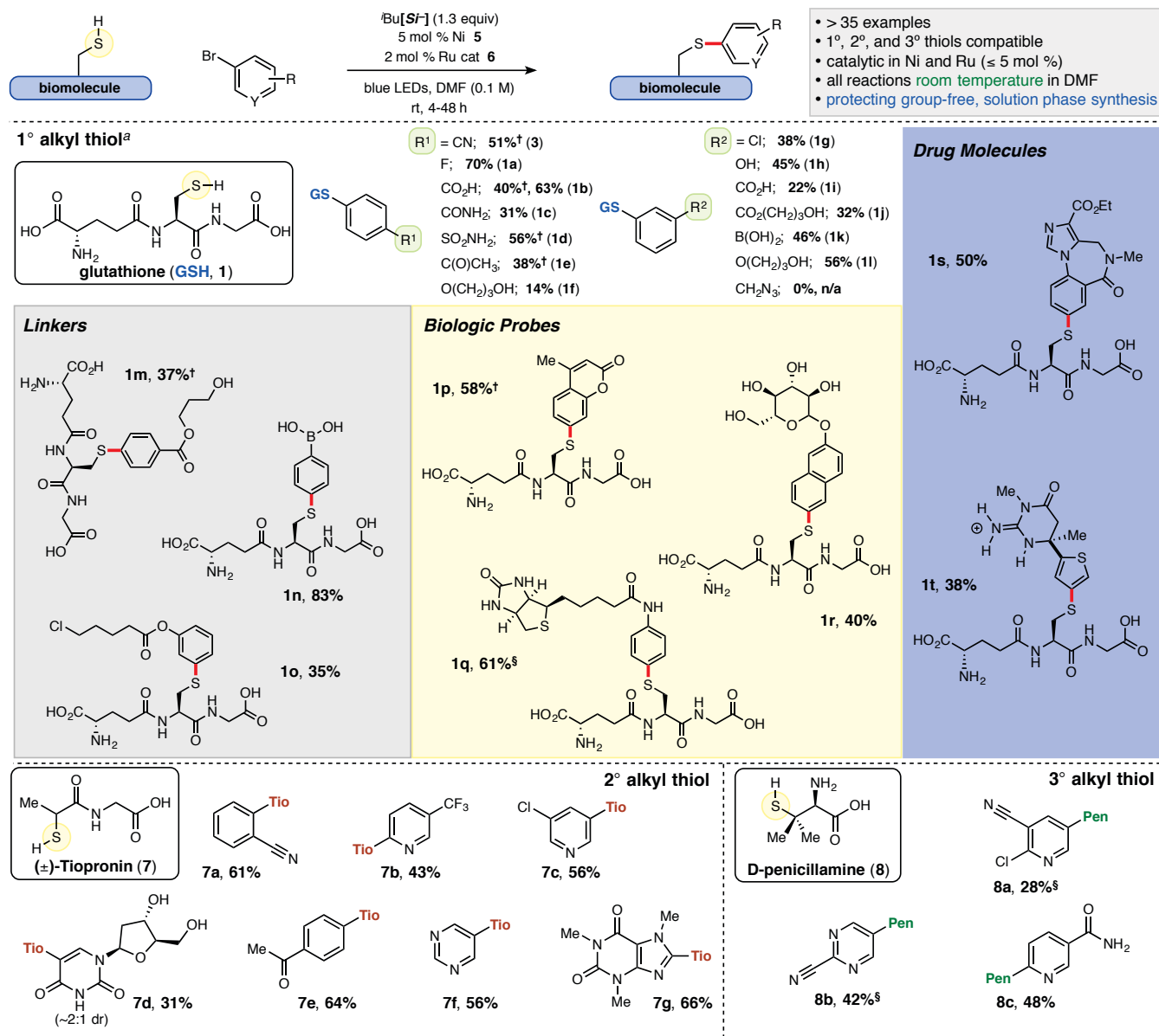
Chart 1. Ni/Photoredox thioarylation reaction and scope of various thiol and arene small molecules. t Bu[Si - ] = diisopropylammonium bis(catechol)isobutylsilicate. DMF = N,N -dimethylformamide. Reactions conducted with 0.1 mmol thiol and ArBr, unless otherwise noted; isolated yields are reported (TFA salt omitted for clarity, see Supporting Information for additional details). a 0.12 mmol GSH employed. § 2 equiv ArBr was employed. † The adduct was filtered following precipitation from the aqueous solution.
