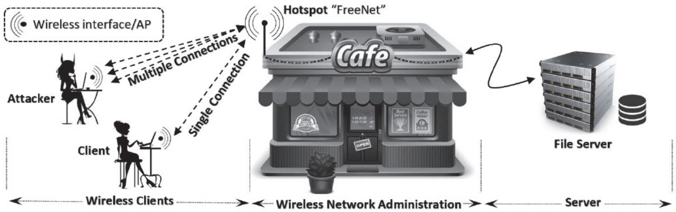
Fig. 2: Proposed attack testbed set up. The attacker and the client used Laptops with TPE-NUSBDB wireless network interface card to connect to the wireless network. Dlink DIR-890L was used as a hotspot and bandwidth controller. We used a Linux based workstation to create the File Server.
