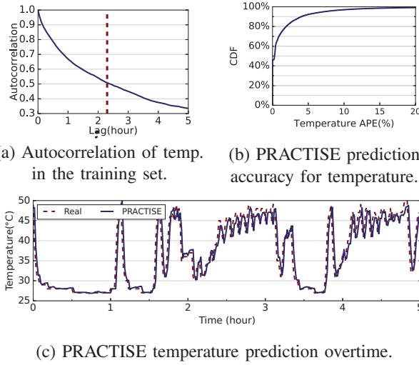
Fig. 9. Autocorrelation and PRACTISE prediction for temperature.
