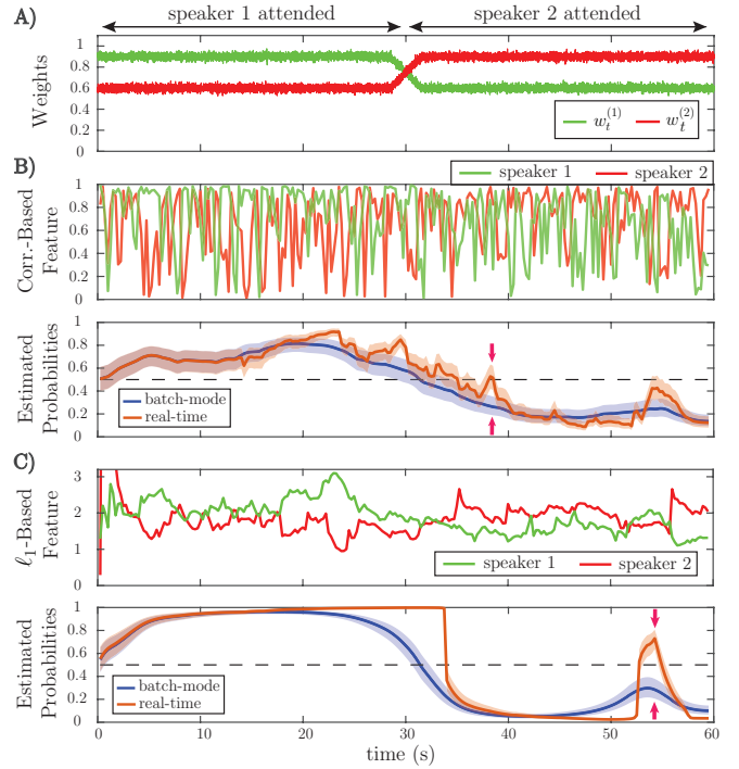
Fig. 3: Results for simulated EEG: A) Input weights w_t^{(1)} and w_t^{(2)} in Eq. (4). B) Outputs of the correlation-based feature and state-space model estimators. C) Outputs of the \ell_1 -based feature and state-space model estimators.
