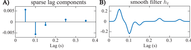
Fig. 2: Impulse response h_t used in Eq. (4): A) sparse lag components, B) the smoothed impulse response.
