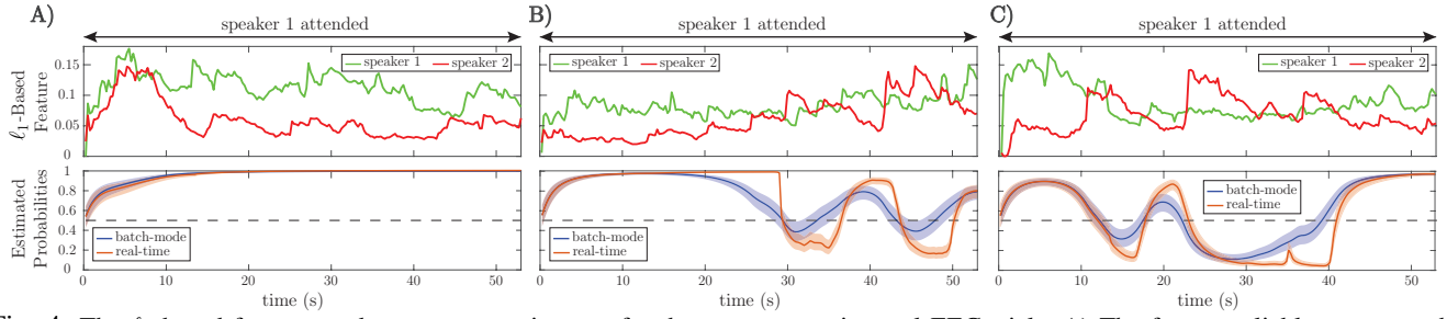
Fig. 4: The \ell_1 -based features and state-space estimators for three representative real EEG trials: A) The feature reliably separates the attended and unattended speakers. B) The feature separates the attended and unattended speakers on average over the trial. C) The feature either fails to separate the two speakers or results in a larger output for the unattended speaker on average, which is unexpected.
