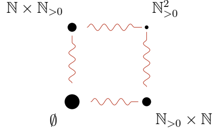
FIGURE 4. Points and topology of \text{Spec } \mathbb{N}^2 . The big point corresponds to the ideal \emptyset , the intermediate points are the primes \mathbb{N} \times \mathbb{N}_{>0} and \mathbb{N}_{>0} \times \mathbb{N} , and the small closed point is the maximal ideal \mathbb{N}_{>0}^2 . The arrow indicate specialization, thus determining the topology.
