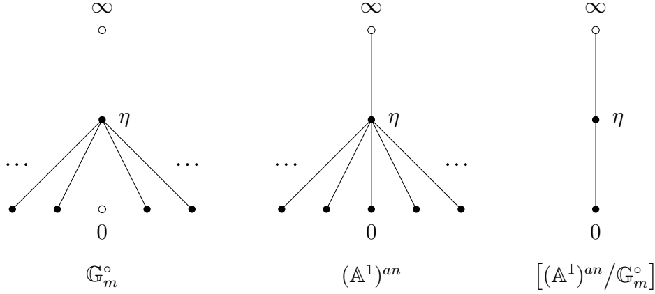
FIGURE 8. Consider the affine line \mathbb{A}^1 over a trivially valued field \mathbf{k} . The non-Archimedean unit circle \mathbb{G}_m^\circ is given as the subset of elements in x \in (\mathbb{A}^1)^{an} with |t|_x = 1 , where t denotes a coordinate on \mathbb{A}^1 . The skeleton \mathfrak{S}(\mathbb{A}^1) of (\mathbb{A}^1)^{an} is the line connecting 0 to \infty . It is precisely the set of " \mathbb{G}_m^\circ -invariant" points in (\mathbb{A}^1)^{an} , and therefore naturally homeomorphic to the topological space underlying [(\mathbb{A}^1)^{an} / \mathbb{G}_m^\circ] (see [Uli14, Example 6.2]).
