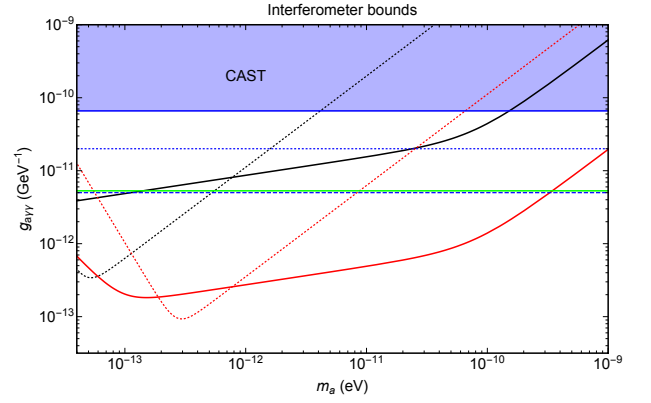
FIG. 5: Same as Fig. 4 but using the configuration shown in Fig. 3. Radiation pressure noise is cancelled leaving only radiation torque noise. We take the beams to be separated by 1 cm and the mirror to be circular and 10 cm in diameter.
