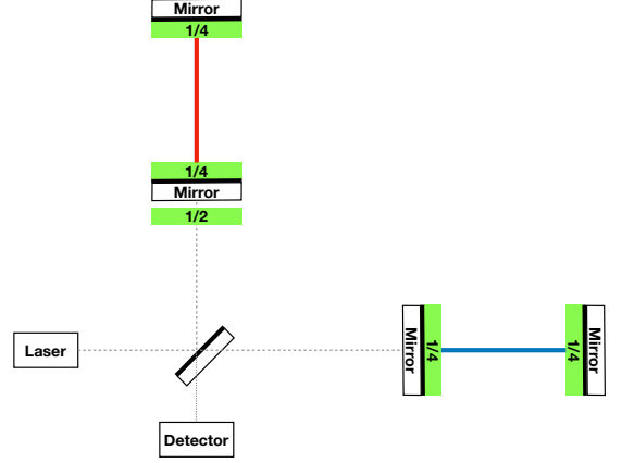
FIG. 2: Diagram of our proposed axion interferometer. It is a standard Michelson interferometer with the additional waveplates necessary to preserve polarization. The two arms of the interferometer both consist of Fabry-Perot cavities that allow the effective path length to be higher than a single-traverse interferometer by roughly a factor of the cavity finesse. The dotted line is linearly polarized light, the red line is \odot polarized light and the blue line is \ominus polarized light. Four quarter waveplates and a half waveplate are used to maintain the circular polarization of the light.
