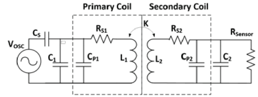
Fig. 1. Wireless Resistive Analog Passive (WRAP) sensor equivalent circuit with parasitic components. R_{Sensor} variation can be probed from the Primary coil voltage ( V_{out} ).
