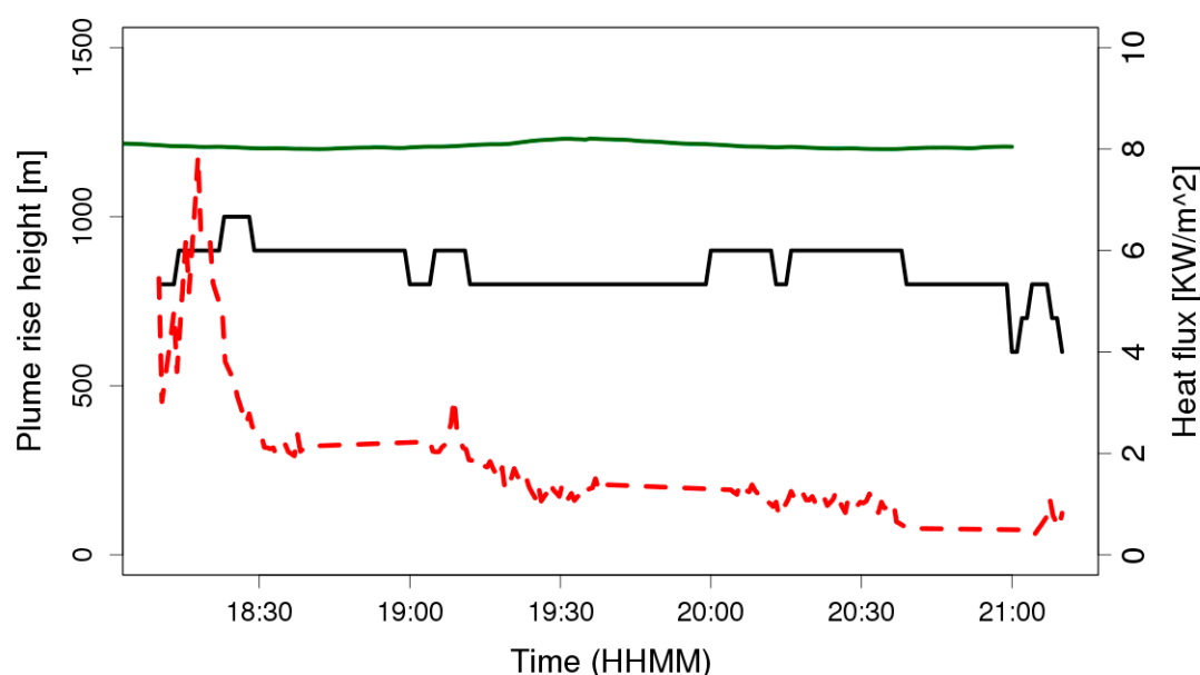
Figure 9. Time series of model-estimated plume rise heights (solid-black line), model-estimated planetary boundary layer (PBL) heights (solid-green line), and fire heat fluxes (red-dashed line) during the L2F prescribed burn.
