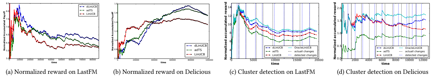
Figure 4: Performance comparison in LastFM &amp; Delicious.
