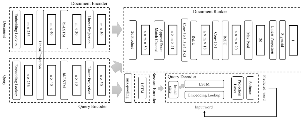
Figure 4: Architecture of the Multi-task Match-Tensor Model (M-Match-Tensor).
