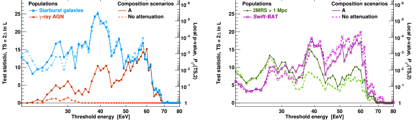
Figure 1. TS scan over the threshold energy for SBGs and AGNs ( Left ) and Swift -BAT and 2MRS sources ( Right ), including attenuation (light-dashed lines) or not (darker-solid lines).
