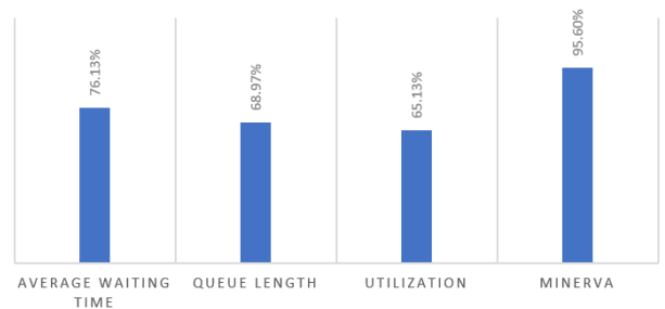
Fig. 7. Comparison of accuracy of bottleneck detection by MINERVA compared to popular bottleneck detection methods for extension of AD05 benchmark
