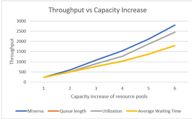
Fig. 8. Line graph for throughput vs increase in resource pool capacity as identified by various bottleneck identification methods for extension of FT06 benchmark
