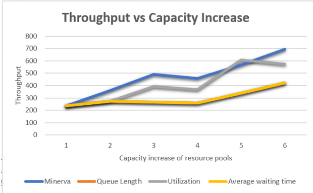
Fig. 9. Line graph for throughput vs increase in resource pool capacity as identified by various bottleneck identification methods for extension of AD05 benchmark
