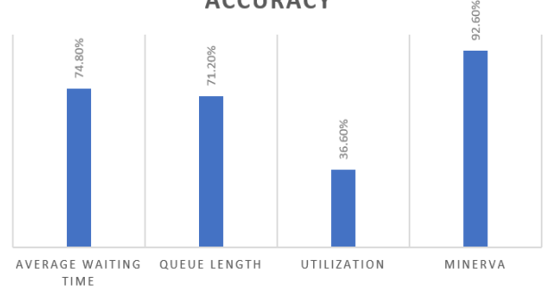
Fig. 5. Comparison of accuracy of bottleneck detection by MINERVA compared to popular bottleneck detection methods for extension of FT06 benchmark
