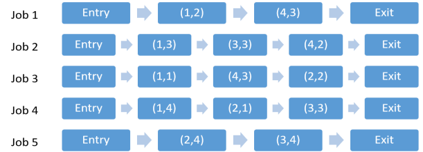
Fig. 6. Figure representing the AD05 JSSP benchmark.
