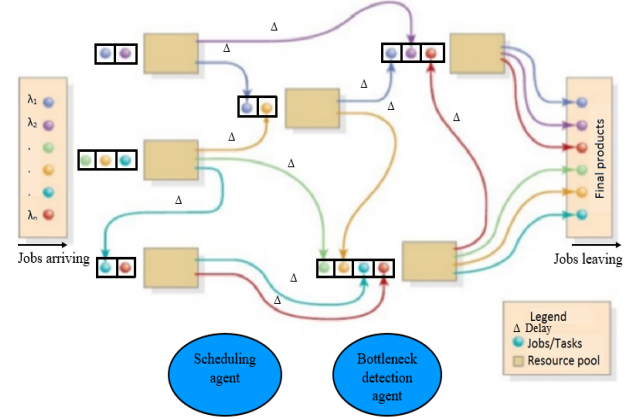
Fig. 1. Schematic of MINERVA
