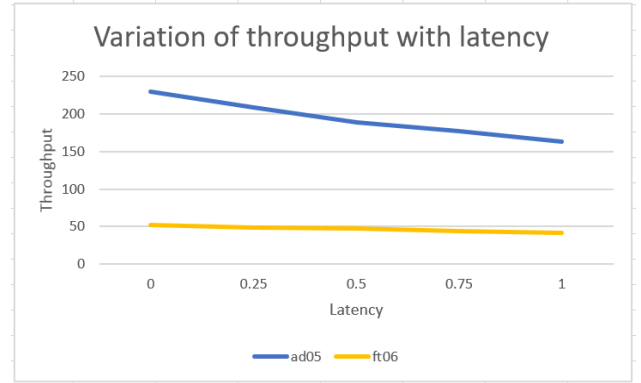
Fig. 10. Line graph for throughput vs latency for extension of FT06 and AD05 benchmarks.
