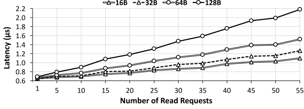
Fig. 7: The average latency of low-load accesses for various request sizes for the number of requests in the range of one to 55.
