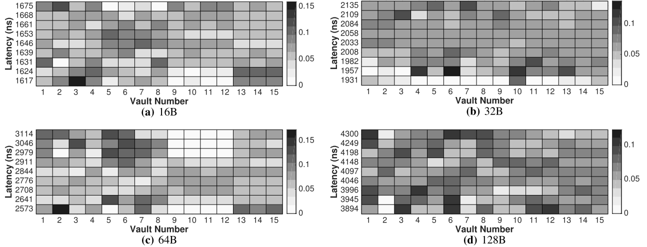
Fig. 12: The vault histograms of each latency interval in heatmaps for various request sizes of (a) 16, (b) 32, (c) 64, and (d) 128 B.
