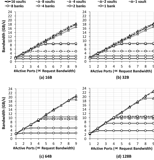
Fig. 13: Relationships between the number of active ports, request bandwidth, and bandwidth for various request sizes.
