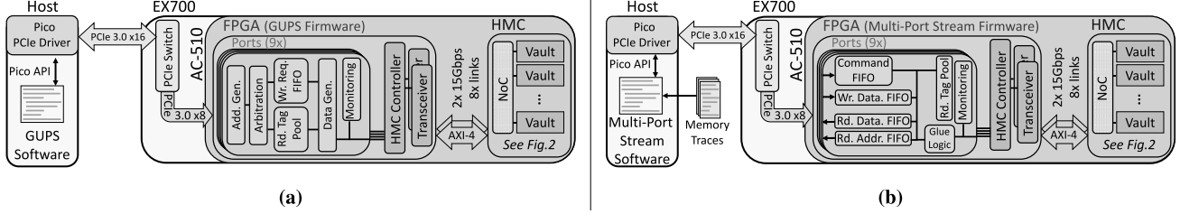
Fig. 5: Firmware and software overview: (a) GUPS and (b) multi-port stream implementations.
