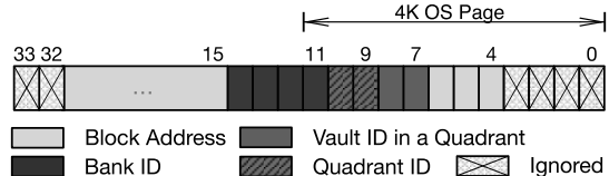
Fig. 3: Address mapping of 4 GB HMC 1.1 with block size of 128 B.
