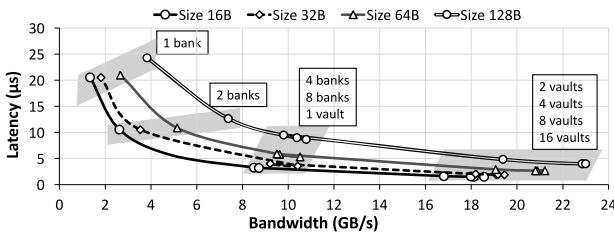
Fig. 6: The relationship between latency and bi-directional bandwidth for various access patterns and request sizes for read-only requests.
