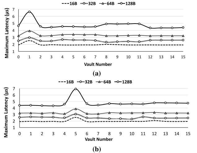
Fig. 9: Maximum observed latency in accessing four vaults, three of which are the same. Accessing vault numbers (a) one (3x) and all vaults; and (b) five (3x) and all vaults. X-axis shows the vault number for the vault that is different.
