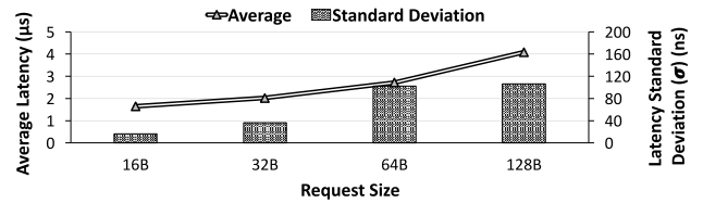
Fig. 11: The average and standard deviation of latency across all vaults for various sizes in the four-vault access pattern.
