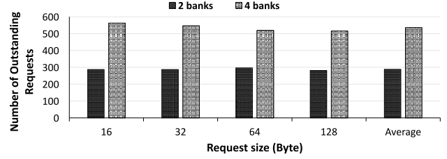
Fig. 14: The number of estimated outstanding requests in two- and four-bank access patterns.
