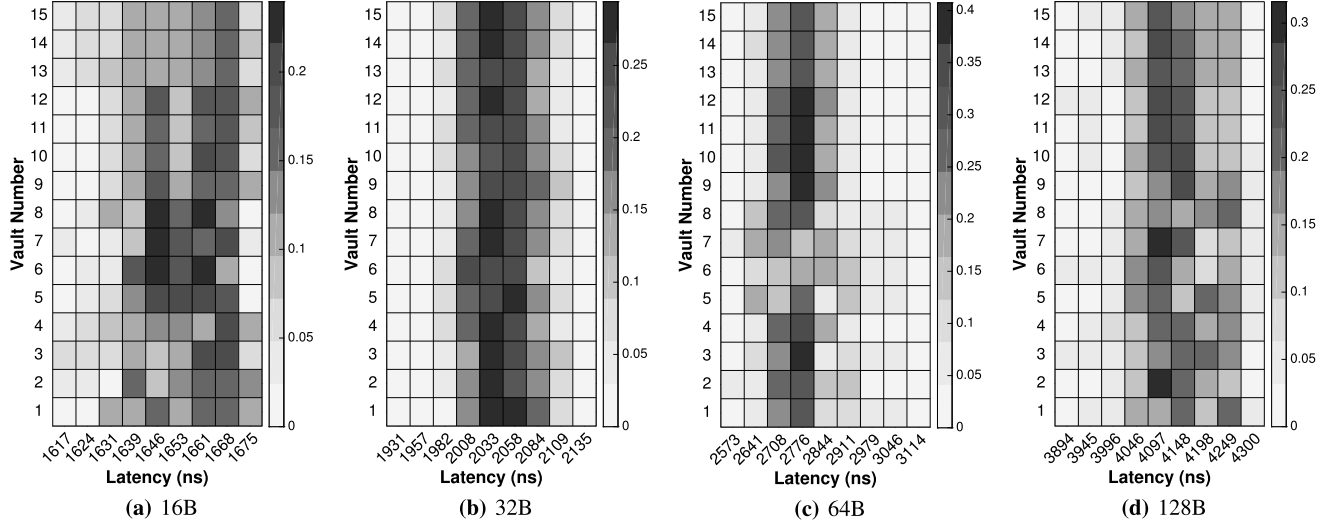
Fig. 10: The latency histograms of each vault in heatmaps for various request sizes of (a) 16, (b) 32, (c) 64, and (d) 128 B.
