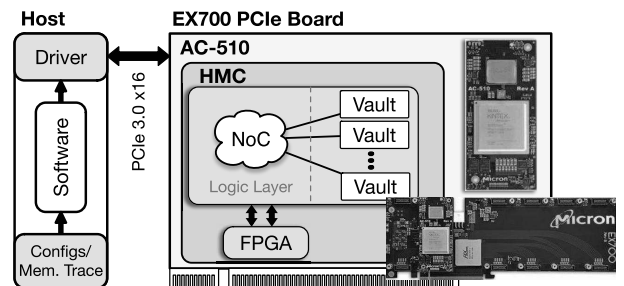
Fig. 1: An overview of our system, and the NoC of the HMC.
