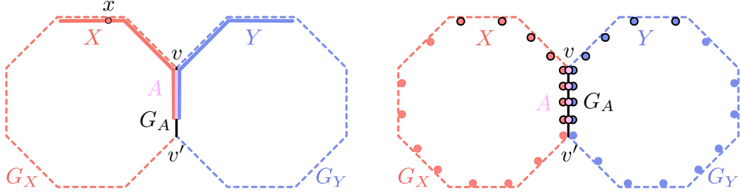
■ Figure 2 Illustration of Theorem 10 on metric graph gluings and both infinite (left) and finite (right) subsets thereof. The metric graphs G_X and G_Y are shown with thin, dotted red and blue lines respectively; X and Y are shown in the infinite case with thick, solid red and blue lines respectively; G_A corresponds to the black solid line while A corresponds to the pink solid line. The finite subset case uses the same color scheme.
