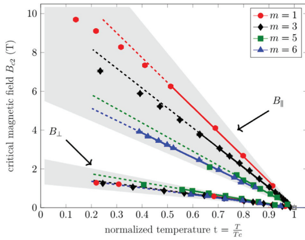
Figure 4. Critical perpendicular magnetic field B_{c\perp}(\text{T}) and critical parallel magnetic field B_{c\parallel}(\text{T}) for [(\text{SnSe})_{1.16}]_m(\text{NbSe}_2)_1 with m = 1, 3, 5 , and 6 . The fits were done according to the Lawrence–Doniach model (equations (3.1) and (3.2)).
