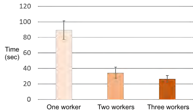
Figure 6: Latency per object in a collaborative setting.
